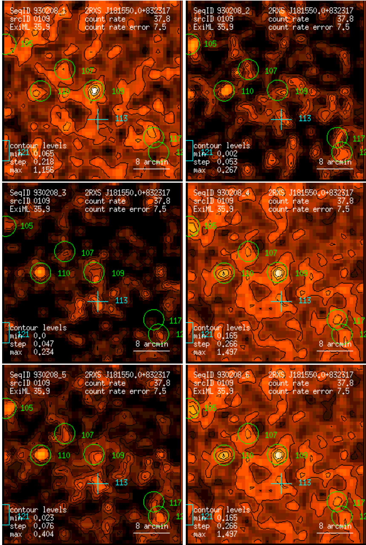
Figure 109: RASS 930208: detection 0109: band rate images, Gaussian filter: (1) PSPC channels 11 – 41, (2) 52 – 90, (3) 91 – 201, (4) 11 – 235, (5) 52 – 201, (6) 11 – 201. Broad band rates in counts/ks. Band rate contour levels in counts/ks/arcmin 2 .
