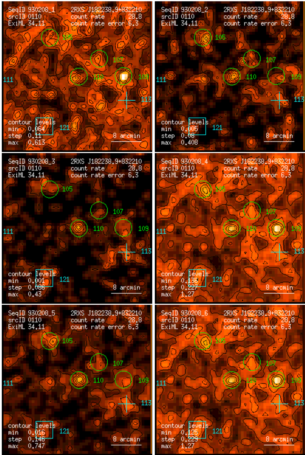
Figure 110: RASS 930208: detection 0110: band rate images, Gaussian filter: (1) PSPC channels 11 – 41, (2) 52 – 90, (3) 91 – 201, (4) 11 – 235, (5) 52 – 201, (6) 11 – 201. Broad band rates in counts/ks. Band rate contour levels in counts/ks/arcmin 2 .
