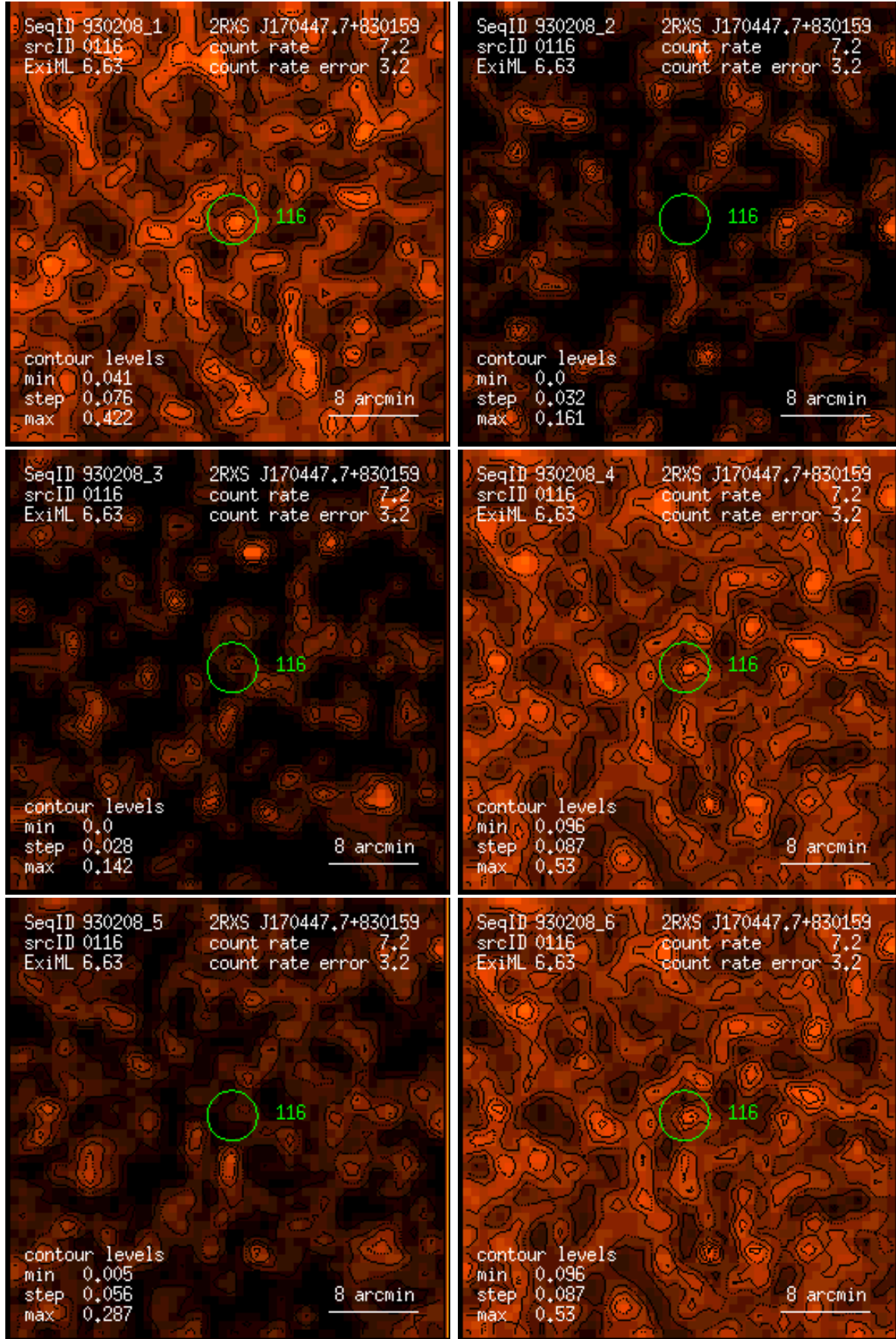
Figure 116: RASS 930208: detection 0116: band rate images, Gaussian filter: (1) PSPC channels 11 – 41, (2) 52 – 90, (3) 91 – 201, (4) 11 – 235, (5) 52 – 201, (6) 11 – 201. Broad band rates in counts/ks. Band rate contour levels in counts/ks/arcmin 2 .
