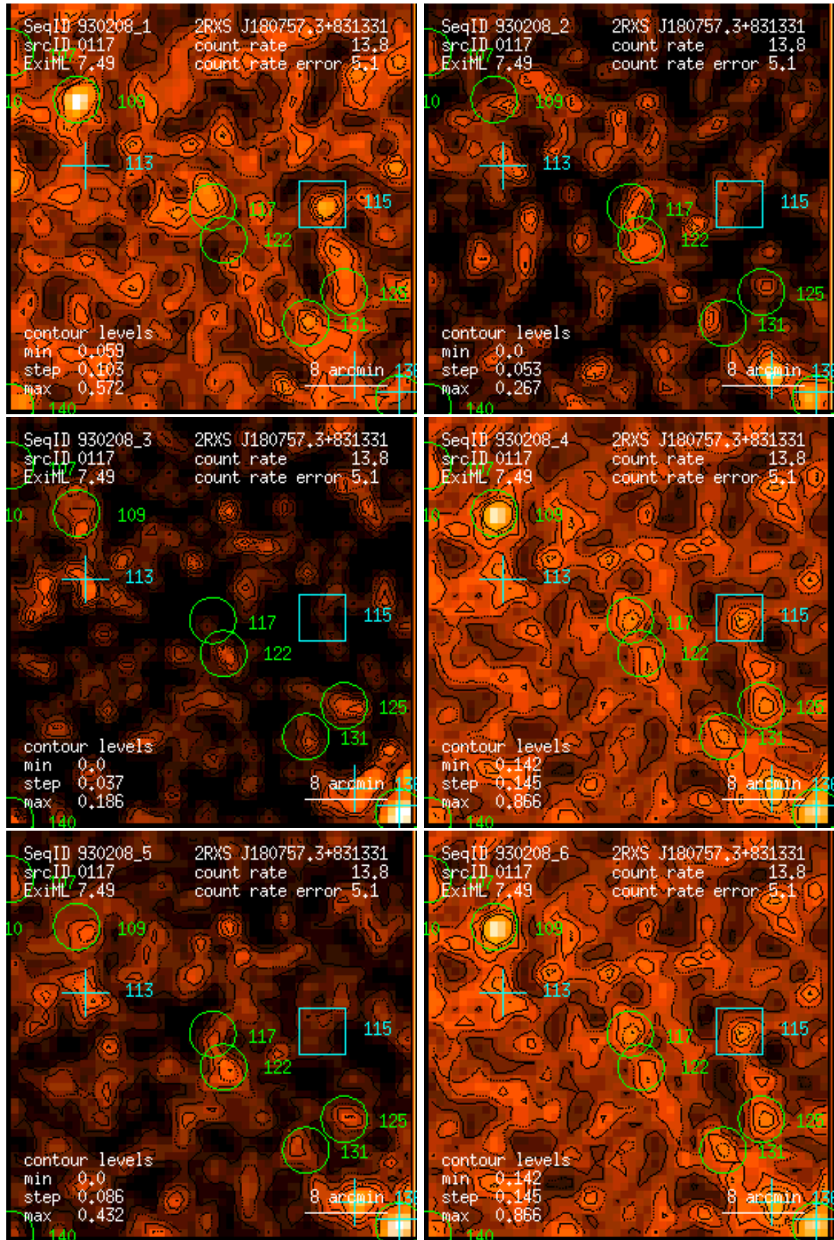
Figure 117: RASS 930208: detection 0117: band rate images, Gaussian filter: (1) PSPC channels 11 – 41, (2) 52 – 90, (3) 91 – 201, (4) 11 – 235, (5) 52 – 201, (6) 11 – 201. Broad band rates in counts/ks. Band rate contour levels in counts/ks/arcmin 2 .
