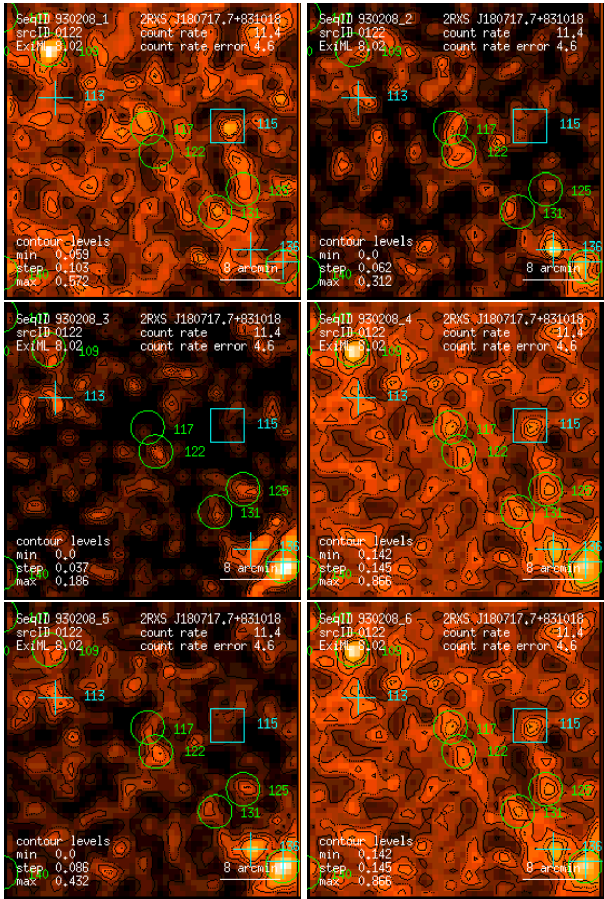
Figure 122: RASS 930208: detection 0122: band rate images, Gaussian filter: (1) PSPC channels 11 – 41, (2) 52 – 90, (3) 91 – 201, (4) 11 – 235, (5) 52 – 201, (6) 11 – 201. Broad band rates in counts/ks. Band rate contour levels in counts/ks/arcmin 2 .
