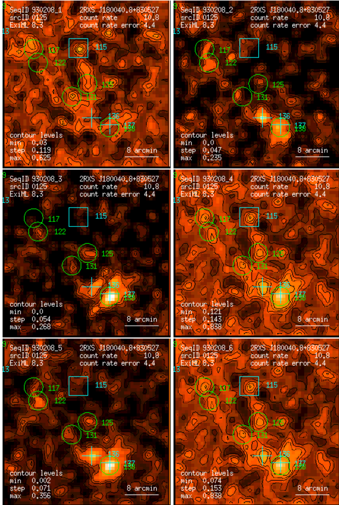
Figure 125: RASS 930208: detection 0125: band rate images, Gaussian filter: (1) PSPC channels 11 – 41, (2) 52 – 90, (3) 91 – 201, (4) 11 – 235, (5) 52 – 201, (6) 11 – 201. Broad band rates in counts/ks. Band rate contour levels in counts/ks/arcmin 2 .
