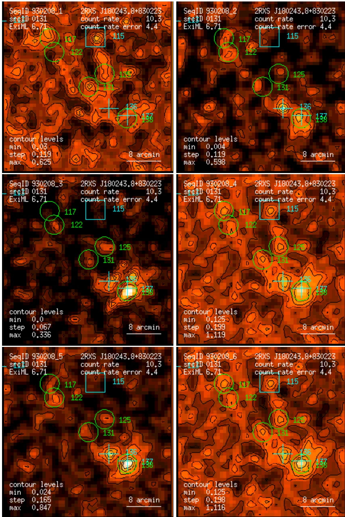
Figure 131: RASS 930208: detection 0131: band rate images, Gaussian filter: (1) PSPC channels 11 – 41, (2) 52 – 90, (3) 91 – 201, (4) 11 – 235, (5) 52 – 201, (6) 11 – 201. Broad band rates in counts/ks. Band rate contour levels in counts/ks/arcmin 2 .
