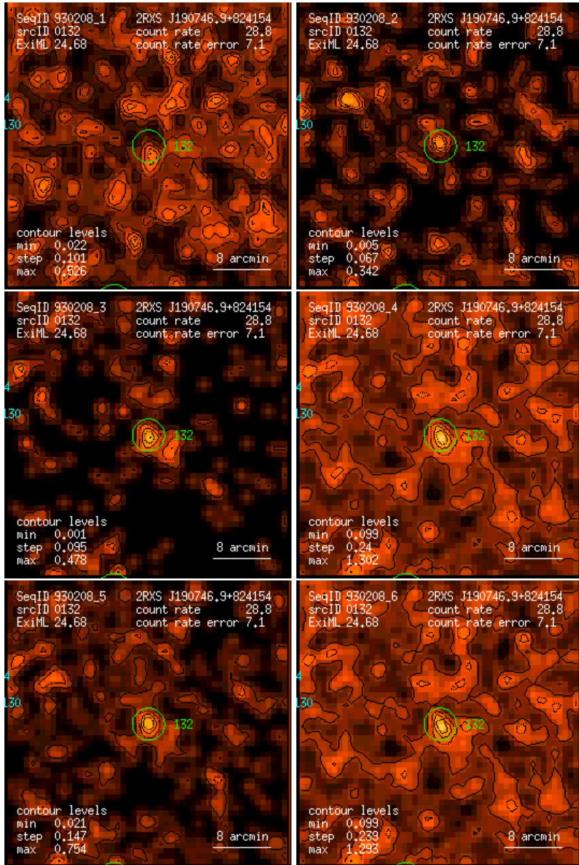
Figure 132: RASS 930208: detection 0132: band rate images, Gaussian filter: (1) PSPC channels 11 – 41, (2) 52 – 90, (3) 91 – 201, (4) 11 – 235, (5) 52 – 201, (6) 11 – 201. Broad band rates in counts/ks. Band rate contour levels in counts/ks/arcmin 2 .
