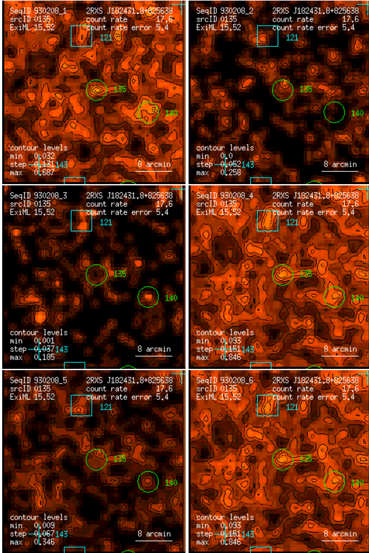
Figure 135: RASS 930208: detection 0135: band rate images, Gaussian filter: (1) PSPC channels 11 – 41, (2) 52 – 90, (3) 91 – 201, (4) 11 – 235, (5) 52 – 201, (6) 11 – 201. Broad band rates in counts/ks. Band rate contour levels in counts/ks/arcmin 2 .
