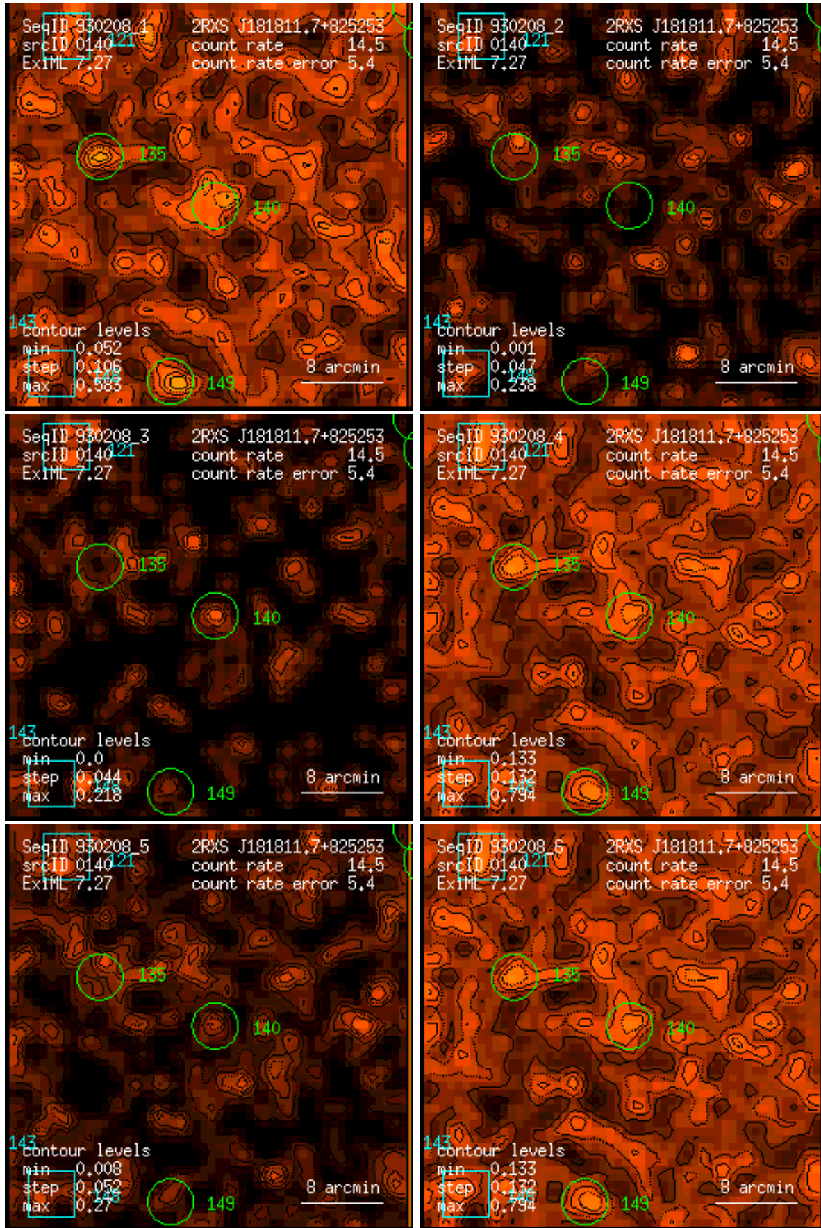
Figure 140: RASS 930208: detection 0140: band rate images, Gaussian filter: (1) PSPC channels 11 – 41, (2) 52 – 90, (3) 91 – 201, (4) 11 – 235, (5) 52 – 201, (6) 11 – 201. Broad band rates in counts/ks. Band rate contour levels in counts/ks/arcmin 2 .
