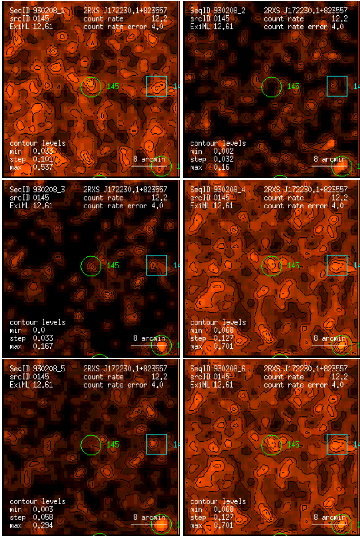
Figure 145: RASS 930208: detection 0145: band rate images, Gaussian filter: (1) PSPC channels 11 – 41, (2) 52 – 90, (3) 91 – 201, (4) 11 – 235, (5) 52 – 201, (6) 11 – 201. Broad band rates in counts/ks. Band rate contour levels in counts/ks/arcmin 2 .
