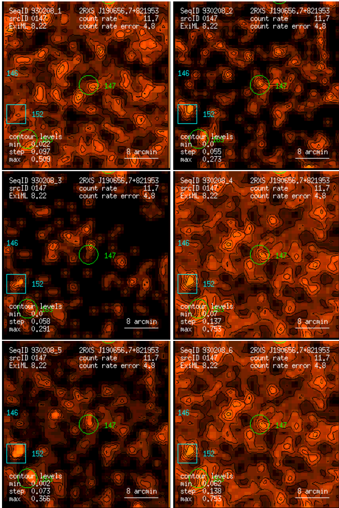
Figure 147: RASS 930208: detection 0147: band rate images, Gaussian filter: (1) PSPC channels 11 – 41, (2) 52 – 90, (3) 91 – 201, (4) 11 – 235, (5) 52 – 201, (6) 11 – 201. Broad band rates in counts/ks. Band rate contour levels in counts/ks/arcmin 2 .
