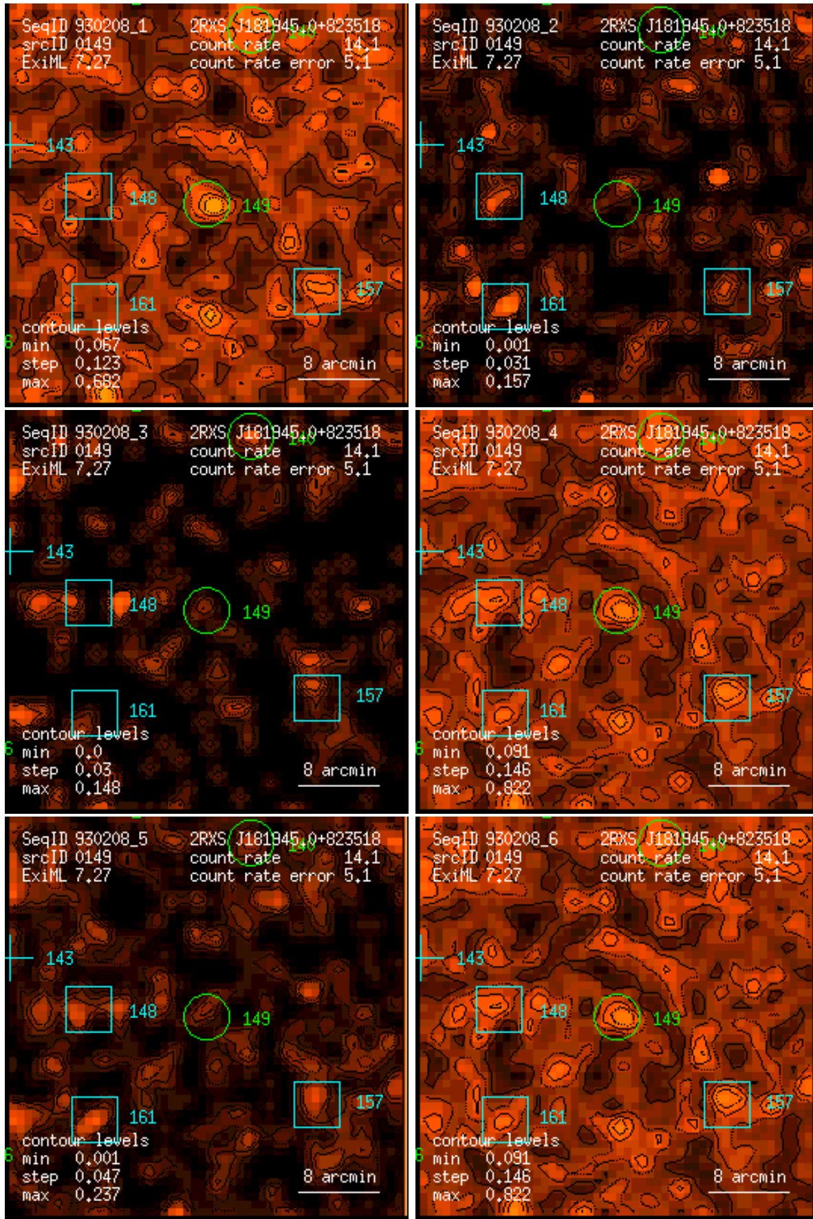
Figure 149: RASS 930208: detection 0149: band rate images, Gaussian filter: (1) PSPC channels 11 – 41, (2) 52 – 90, (3) 91 – 201, (4) 11 – 235, (5) 52 – 201, (6) 11 – 201. Broad band rates in counts/ks. Band rate contour levels in counts/ks/arcmin 2 .
