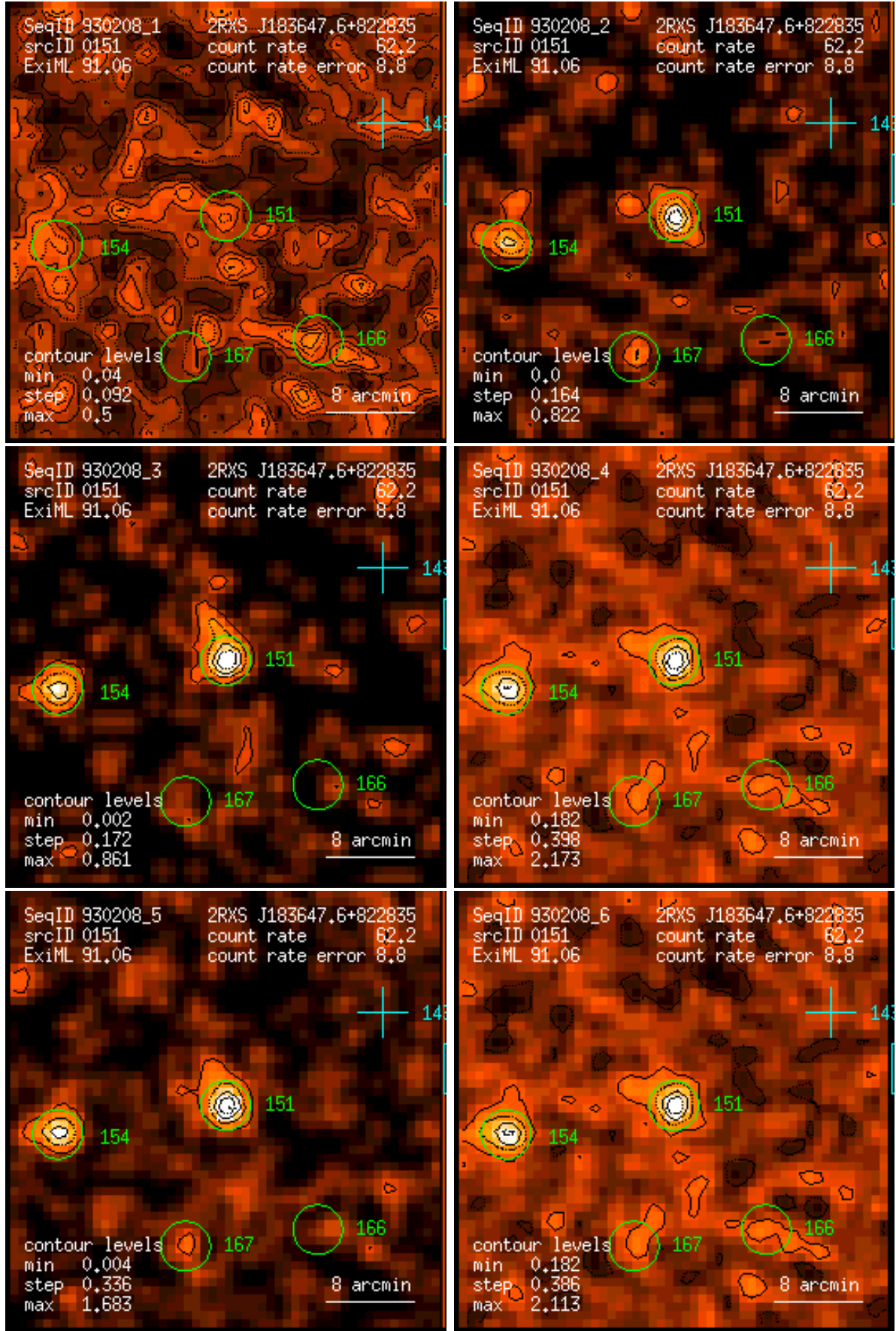
Figure 151: RASS 930208: detection 0151: band rate images, Gaussian filter: (1) PSPC channels 11 – 41, (2) 52 – 90, (3) 91 – 201, (4) 11 – 235, (5) 52 – 201, (6) 11 – 201. Broad band rates in counts/ks. Band rate contour levels in counts/ks/arcmin 2 .
