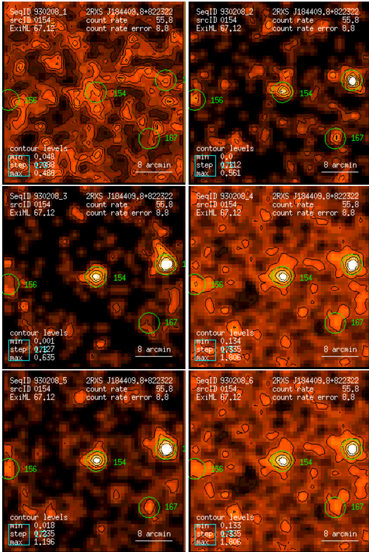
Figure 154: RASS 930208: detection 0154: band rate images, Gaussian filter: (1) PSPC channels 11 – 41, (2) 52 – 90, (3) 91 – 201, (4) 11 – 235, (5) 52 – 201, (6) 11 – 201. Broad band rates in counts/ks. Band rate contour levels in counts/ks/arcmin 2 .
