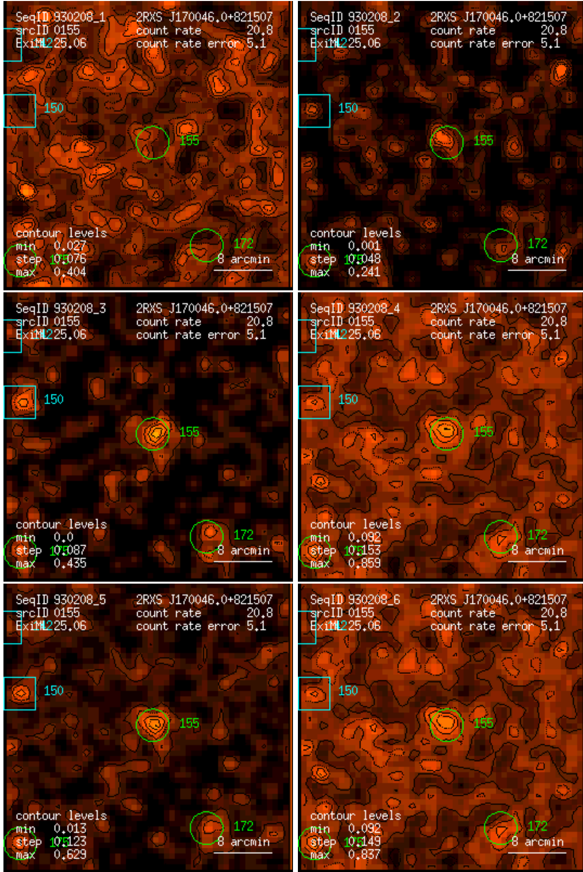
Figure 155: RASS 930208: detection 0155: band rate images, Gaussian filter: (1) PSPC channels 11 – 41, (2) 52 – 90, (3) 91 – 201, (4) 11 – 235, (5) 52 – 201, (6) 11 – 201. Broad band rates in counts/ks. Band rate contour levels in counts/ks/arcmin 2 .
