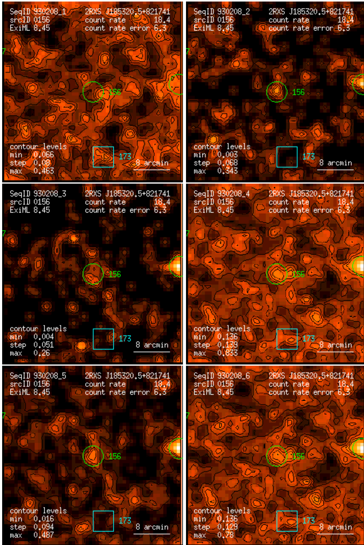
Figure 156: RASS 930208: detection 0156: band rate images, Gaussian filter: (1) PSPC channels 11 – 41, (2) 52 – 90, (3) 91 – 201, (4) 11 – 235, (5) 52 – 201, (6) 11 – 201. Broad band rates in counts/ks. Band rate contour levels in counts/ks/arcmin 2 .
