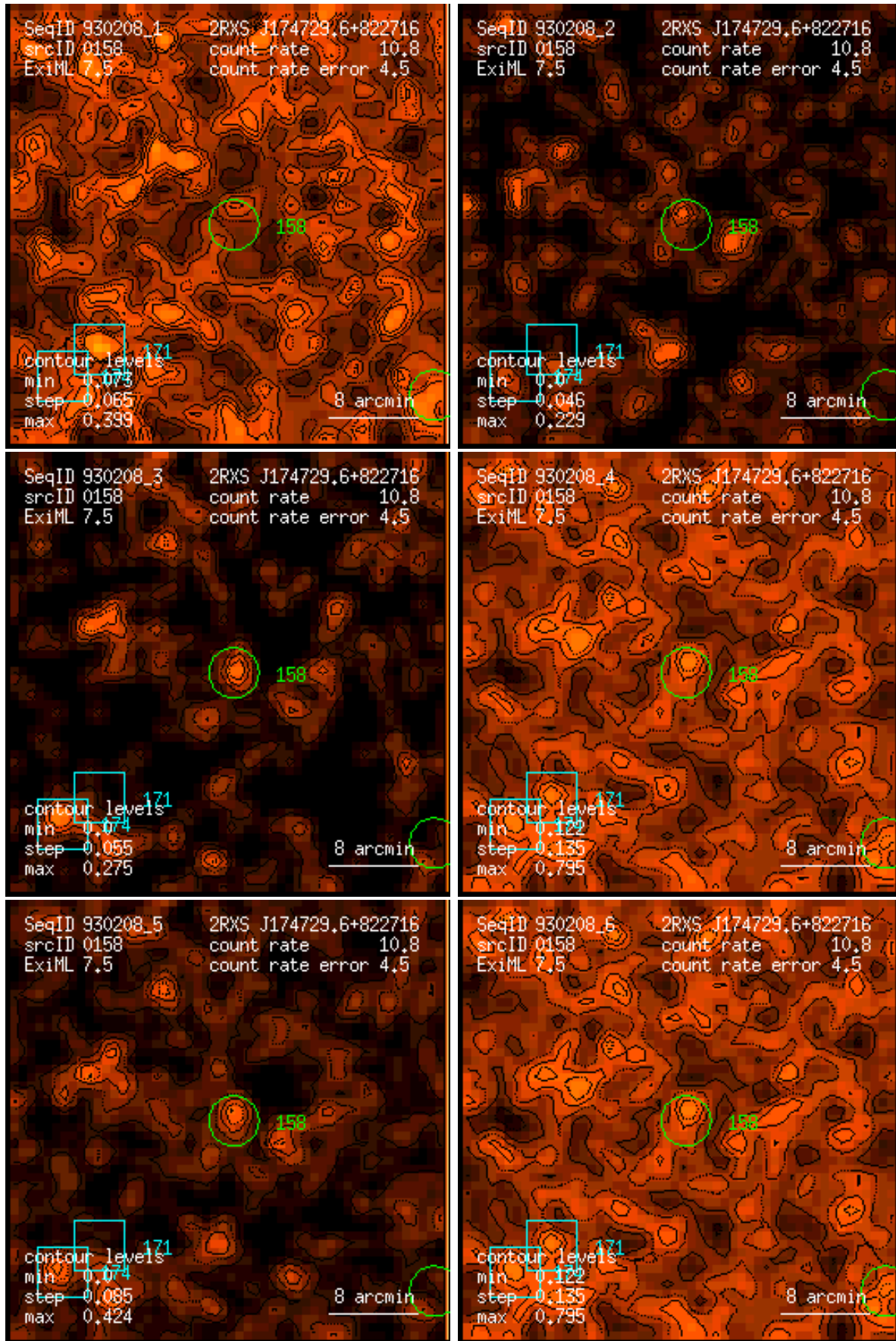
Figure 158: RASS 930208: detection 0158: band rate images, Gaussian filter: (1) PSPC channels 11 – 41, (2) 52 – 90, (3) 91 – 201, (4) 11 – 235, (5) 52 – 201, (6) 11 – 201. Broad band rates in counts/ks. Band rate contour levels in counts/ks/arcmin 2 .
