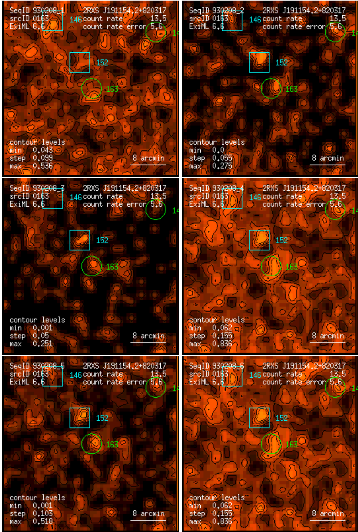
Figure 163: RASS 930208: detection 0163: band rate images, Gaussian filter: (1) PSPC channels 11 – 41, (2) 52 – 90, (3) 91 – 201, (4) 11 – 235, (5) 52 – 201, (6) 11 – 201. Broad band rates in counts/ks. Band rate contour levels in counts/ks/arcmin 2 .
