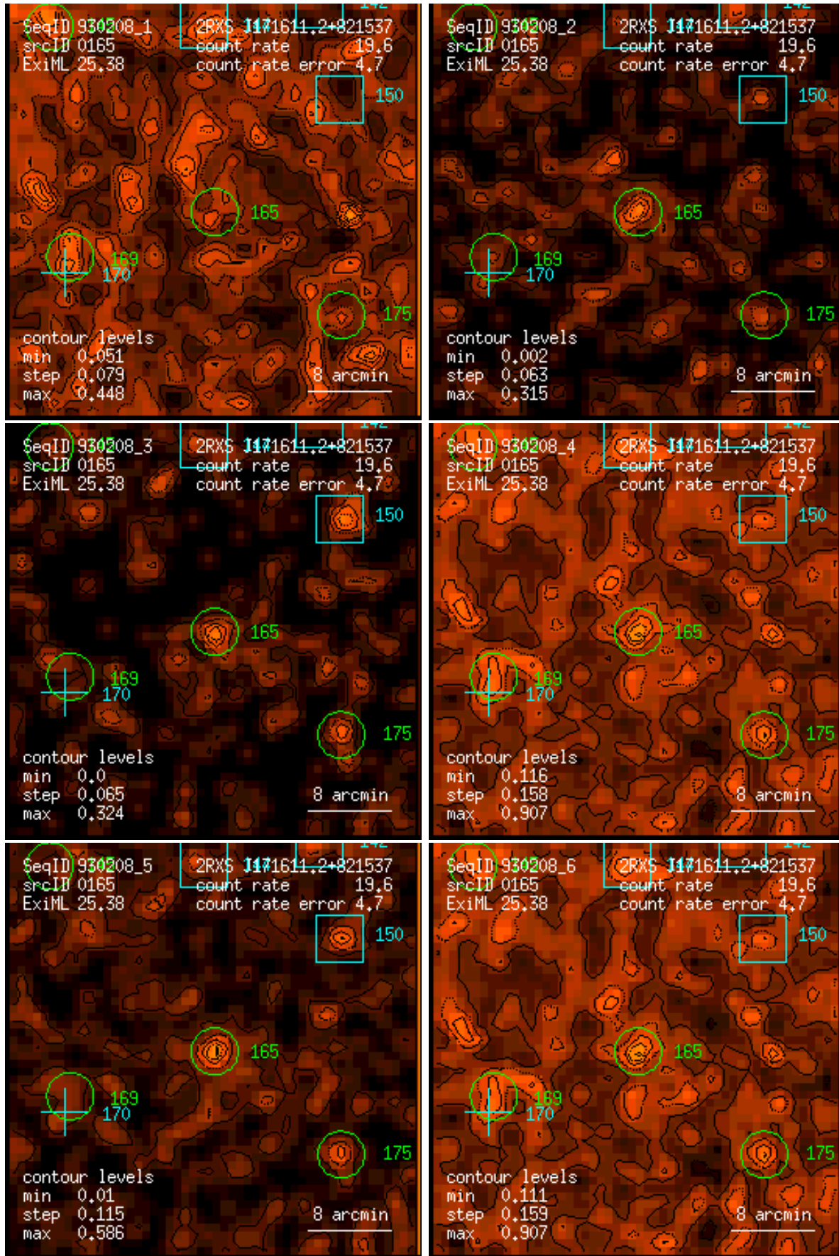
Figure 165: RASS 930208: detection 0165: band rate images, Gaussian filter: (1) PSPC channels 11 – 41, (2) 52 – 90, (3) 91 – 201, (4) 11 – 235, (5) 52 – 201, (6) 11 – 201. Broad band rates in counts/ks. Band rate contour levels in counts/ks/arcmin 2 .
