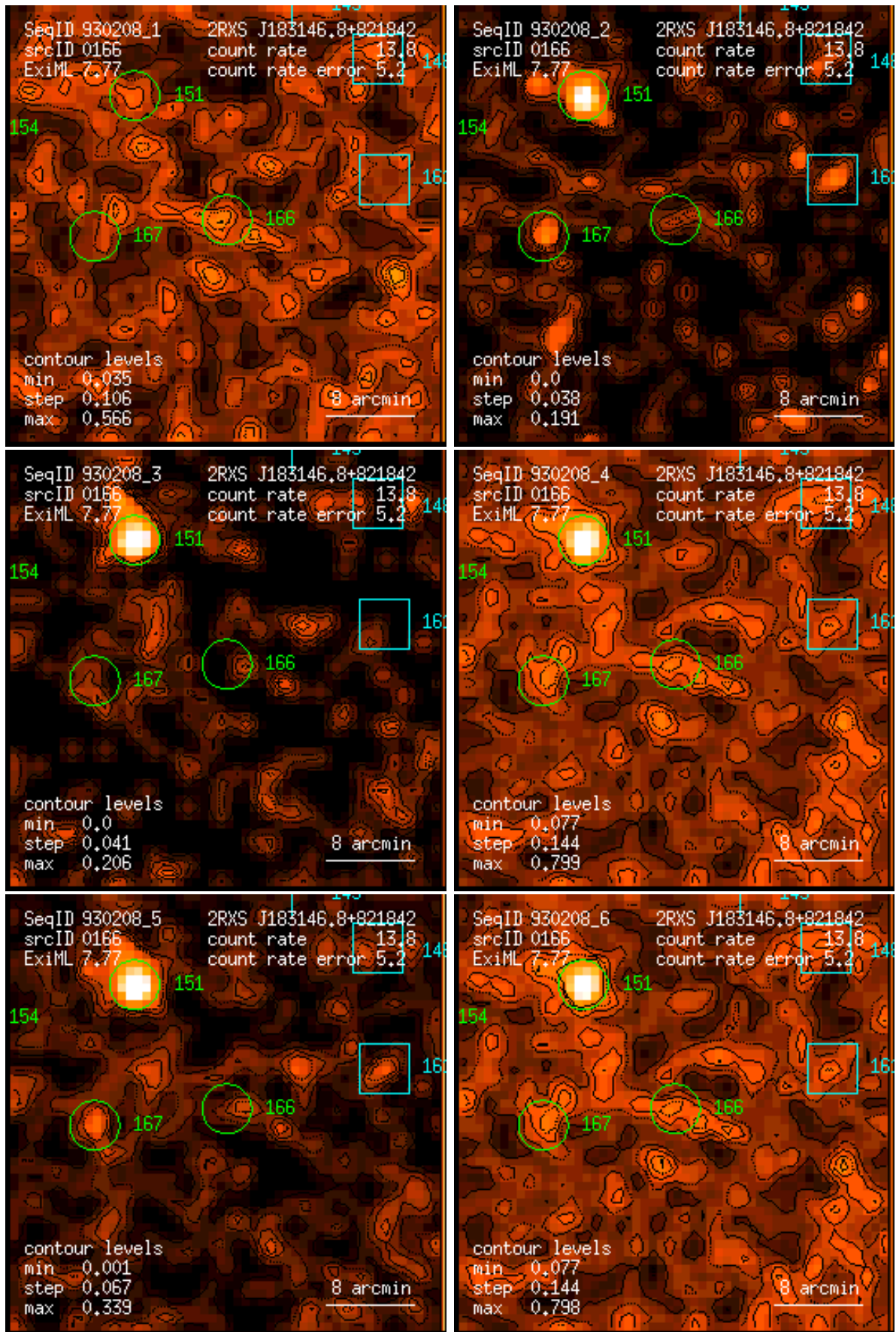
Figure 166: RASS 930208: detection 0166: band rate images, Gaussian filter: (1) PSPC channels 11 – 41, (2) 52 – 90, (3) 91 – 201, (4) 11 – 235, (5) 52 – 201, (6) 11 – 201. Broad band rates in counts/ks. Band rate contour levels in counts/ks/arcmin 2 .
