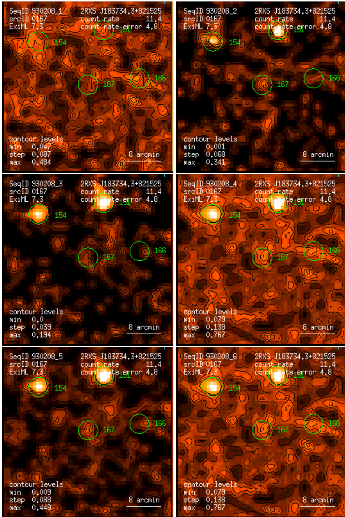
Figure 167: RASS 930208: detection 0167: band rate images, Gaussian filter: (1) PSPC channels 11 – 41, (2) 52 – 90, (3) 91 – 201, (4) 11 – 235, (5) 52 – 201, (6) 11 – 201. Broad band rates in counts/ks. Band rate contour levels in counts/ks/arcmin 2 .
