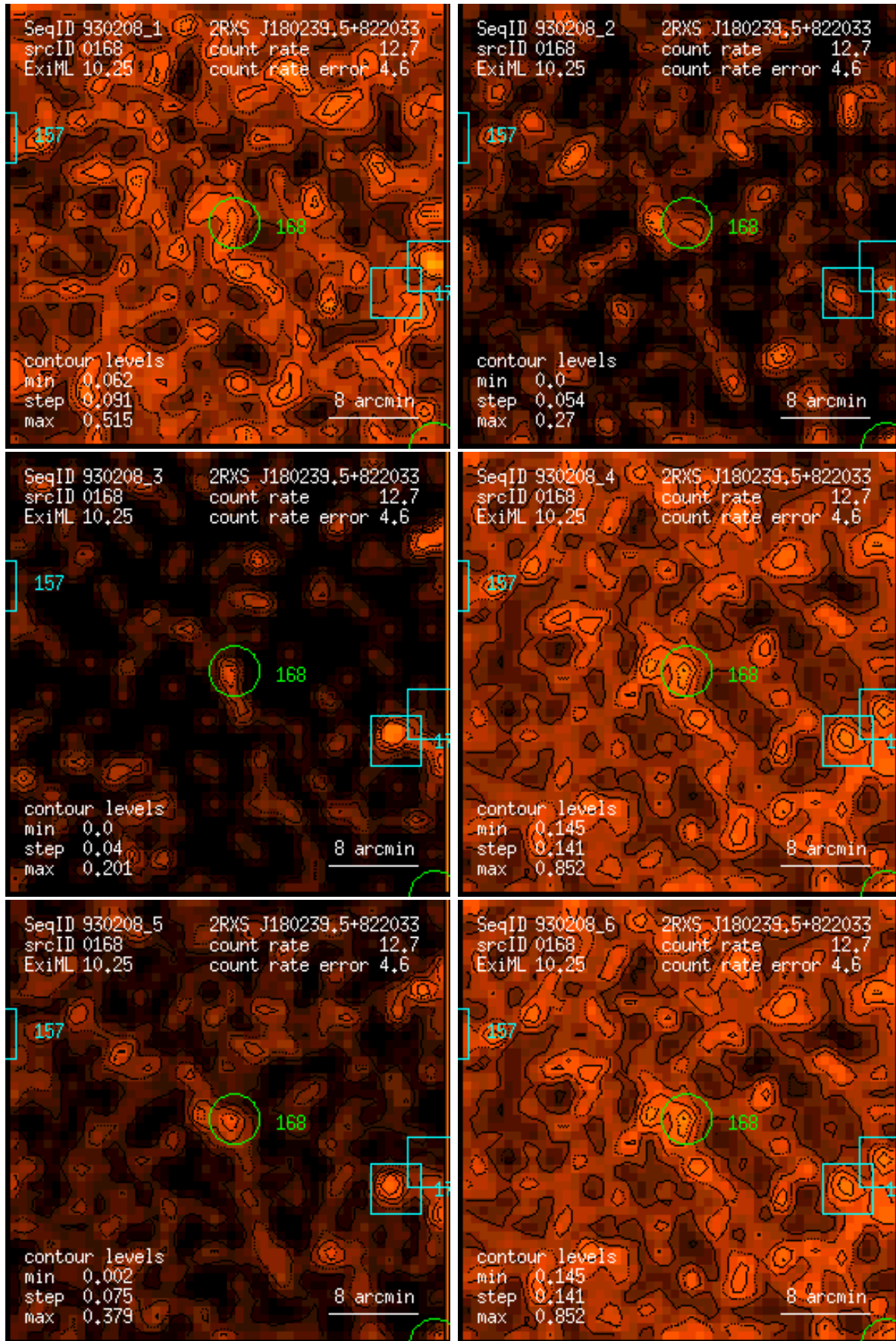
Figure 168: RASS 930208: detection 0168: band rate images, Gaussian filter: (1) PSPC channels 11 – 41, (2) 52 – 90, (3) 91 – 201, (4) 11 – 235, (5) 52 – 201, (6) 11 – 201. Broad band rates in counts/ks. Band rate contour levels in counts/ks/arcmin 2 .
