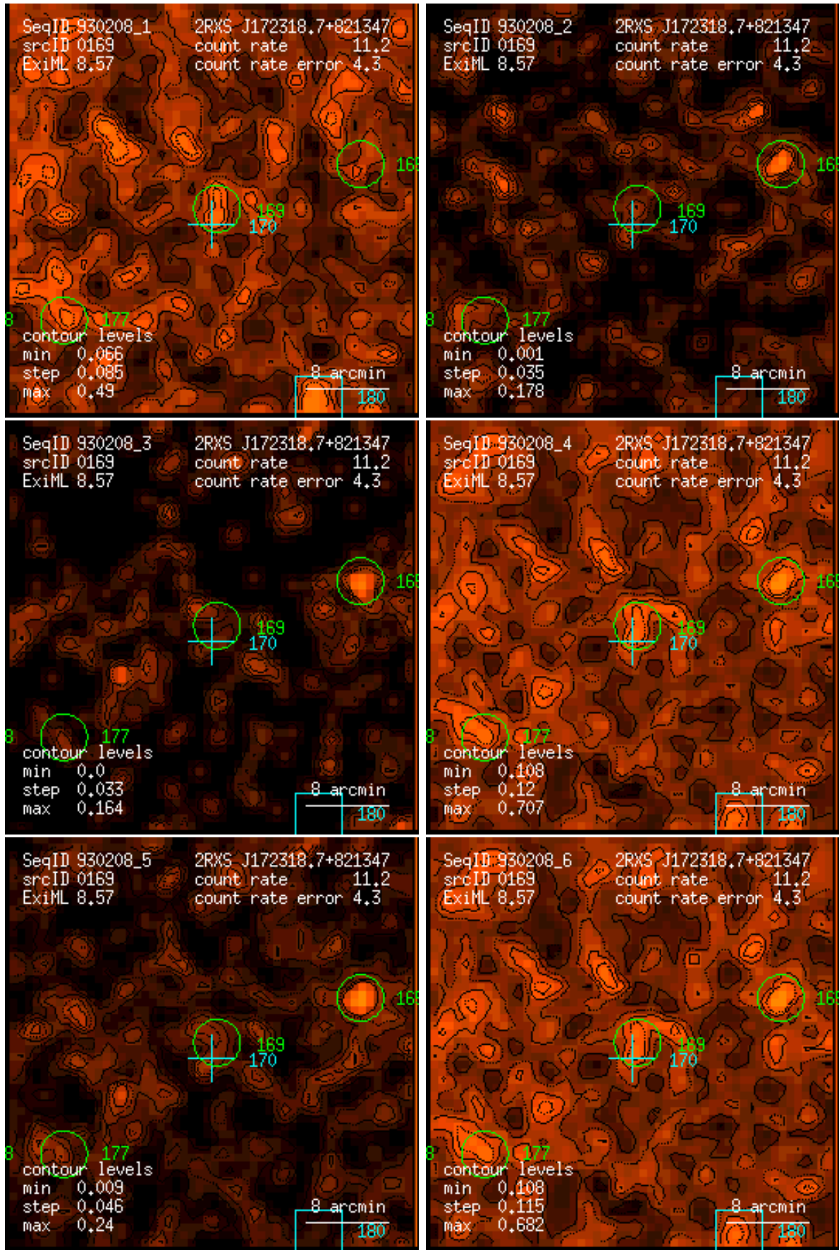
Figure 169: RASS 930208: detection 0169: band rate images, Gaussian filter: (1) PSPC channels 11 – 41, (2) 52 – 90, (3) 91 – 201, (4) 11 – 235, (5) 52 – 201, (6) 11 – 201. Broad band rates in counts/ks. Band rate contour levels in counts/ks/arcmin 2 .
