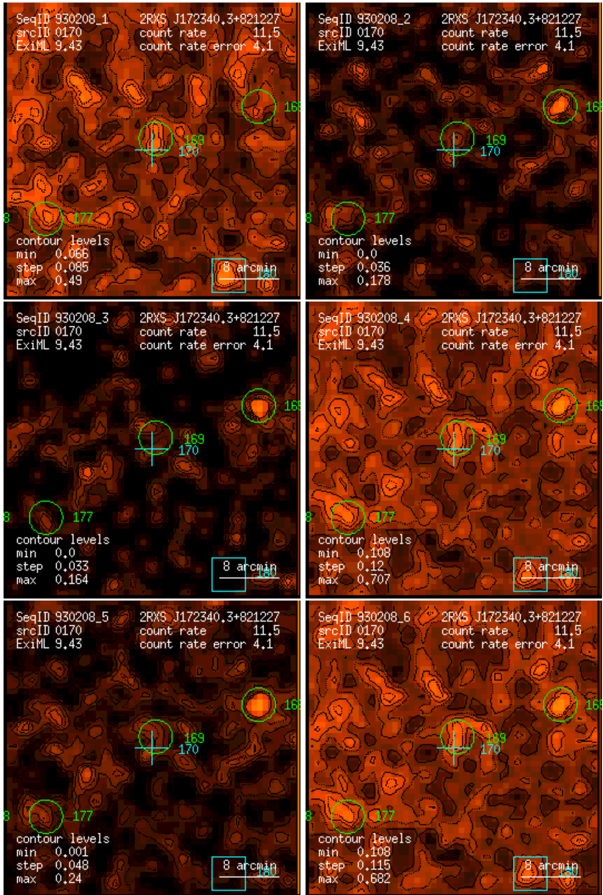
Figure 170: RASS 930208: detection 0170: band rate images, Gaussian filter: (1) PSPC channels 11 – 41, (2) 52 – 90, (3) 91 – 201, (4) 11 – 235, (5) 52 – 201, (6) 11 – 201. Broad band rates in counts/ks. Band rate contour levels in counts/ks/arcmin 2 .
