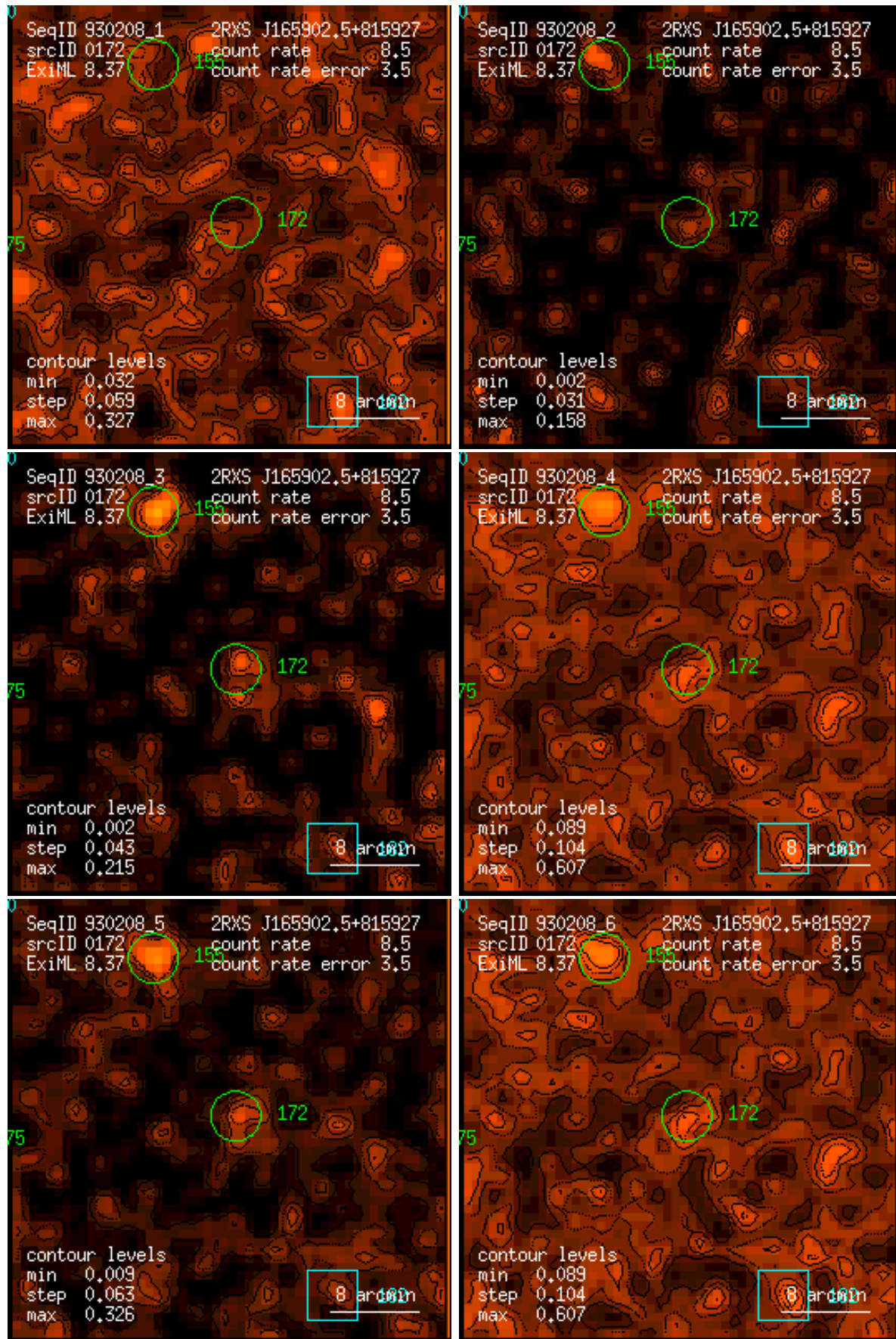
Figure 172: RASS 930208: detection 0172: band rate images, Gaussian filter: (1) PSPC channels 11 – 41, (2) 52 – 90, (3) 91 – 201, (4) 11 – 235, (5) 52 – 201, (6) 11 – 201. Broad band rates in counts/ks. Band rate contour levels in counts/ks/arcmin 2 .
