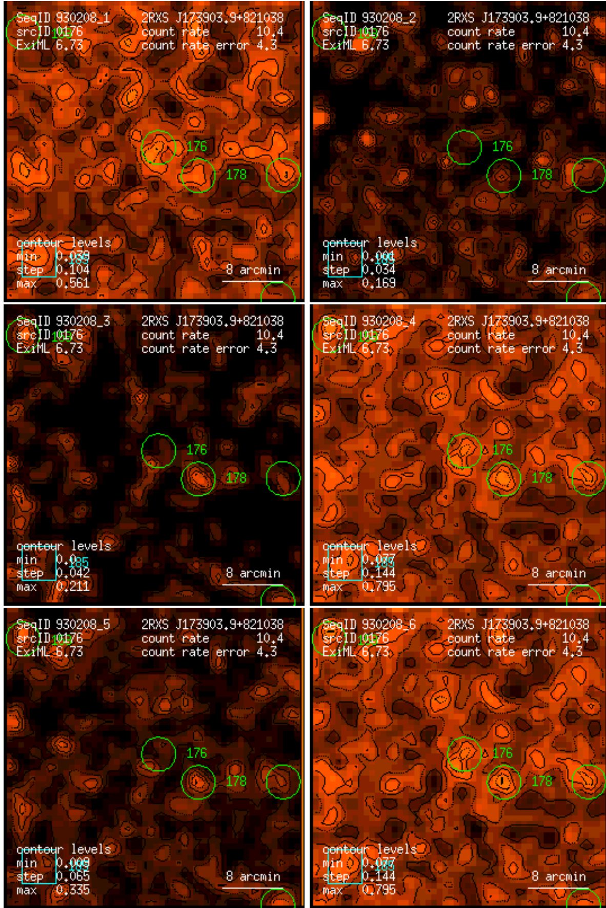
Figure 176: RASS 930208: detection 0176: band rate images, Gaussian filter: (1) PSPC channels 11 – 41, (2) 52 – 90, (3) 91 – 201, (4) 11 – 235, (5) 52 – 201, (6) 11 – 201. Broad band rates in counts/ks. Band rate contour levels in counts/ks/arcmin 2 .
