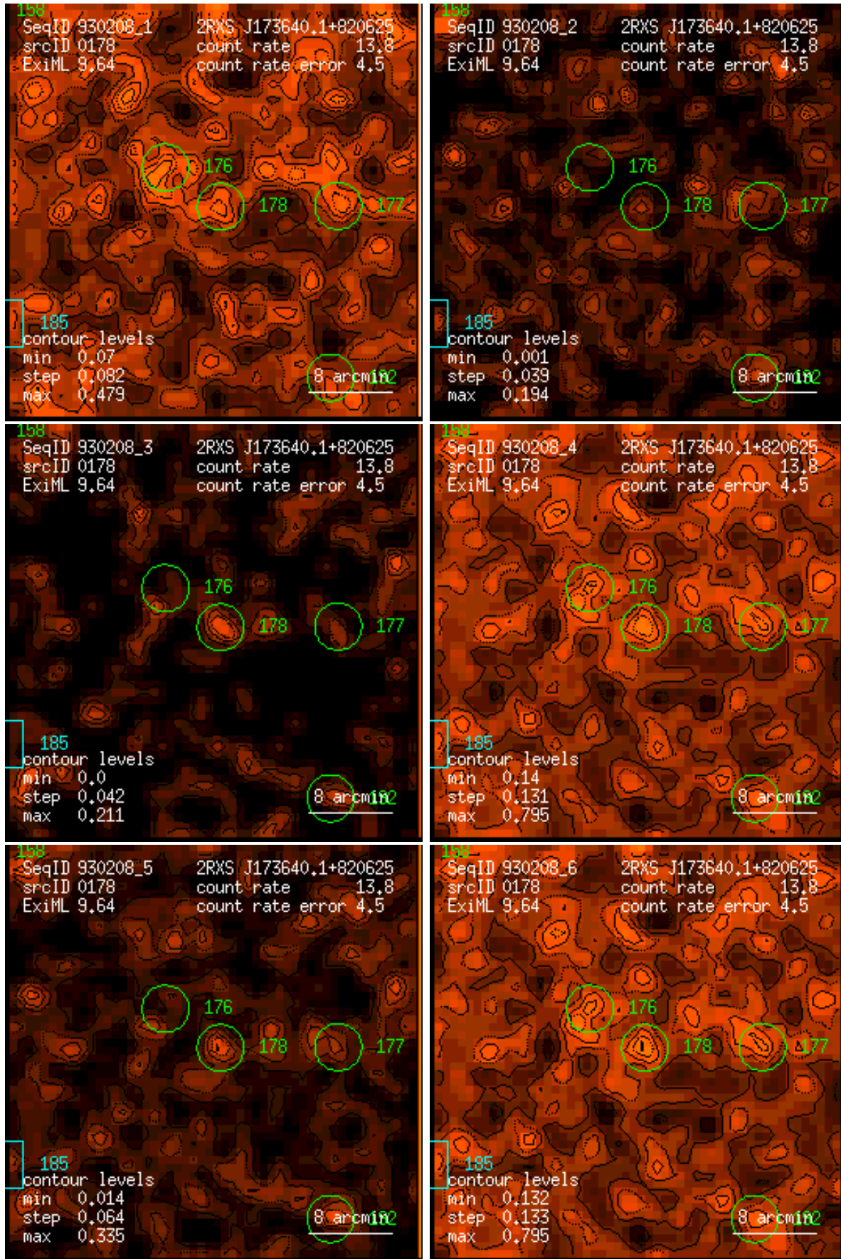
Figure 178: RASS 930208: detection 0178: band rate images, Gaussian filter: (1) PSPC channels 11 – 41, (2) 52 – 90, (3) 91 – 201, (4) 11 – 235, (5) 52 – 201, (6) 11 – 201. Broad band rates in counts/ks. Band rate contour levels in counts/ks/arcmin 2 .
