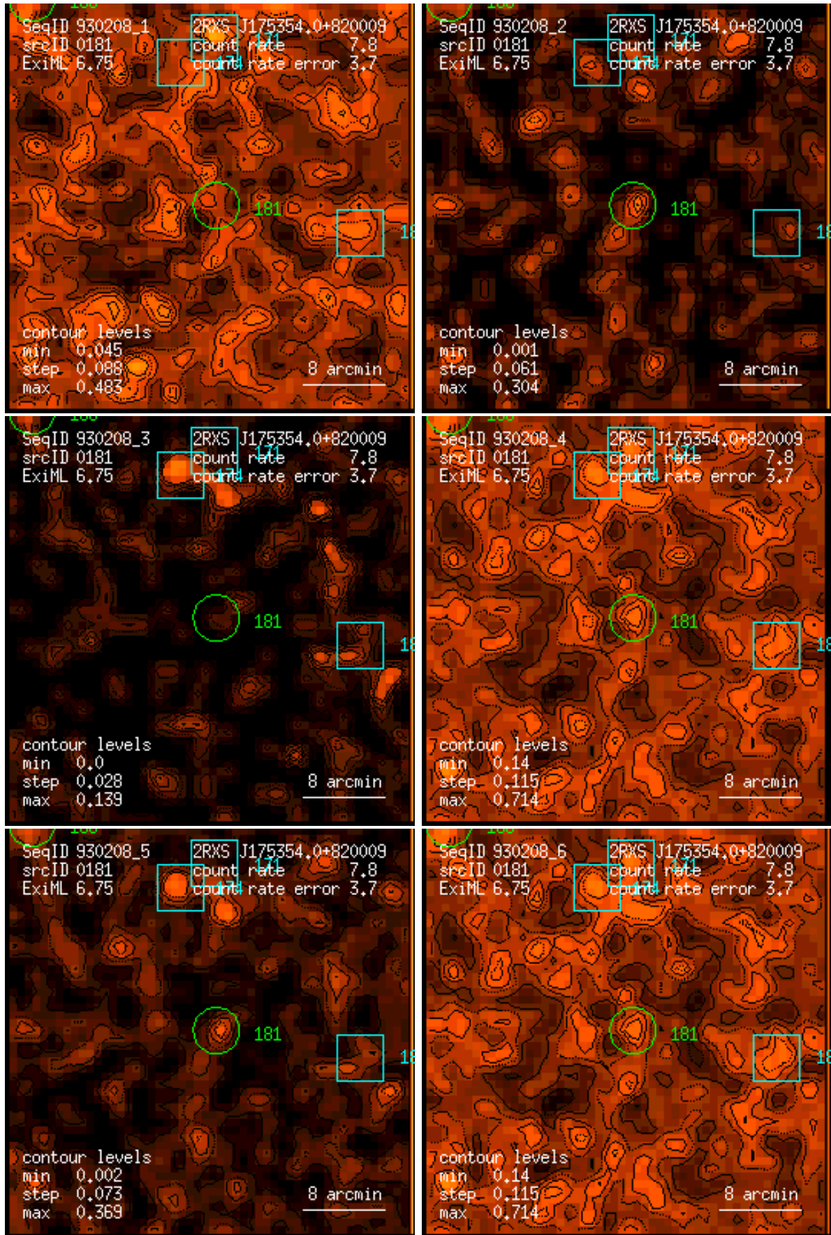
Figure 181: RASS 930208: detection 0181: band rate images, Gaussian filter: (1) PSPC channels 11 – 41, (2) 52 – 90, (3) 91 – 201, (4) 11 – 235, (5) 52 – 201, (6) 11 – 201. Broad band rates in counts/ks. Band rate contour levels in counts/ks/arcmin 2 .
