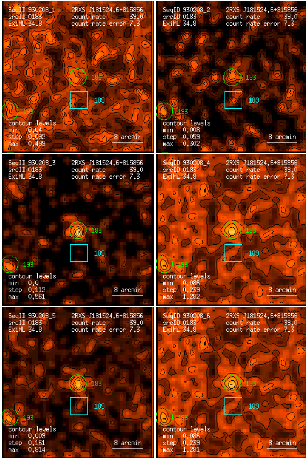
Figure 183: RASS 930208: detection 0183: band rate images, Gaussian filter: (1) PSPC channels 11 – 41, (2) 52 – 90, (3) 91 – 201, (4) 11 – 235, (5) 52 – 201, (6) 11 – 201. Broad band rates in counts/ks. Band rate contour levels in counts/ks/arcmin 2 .
