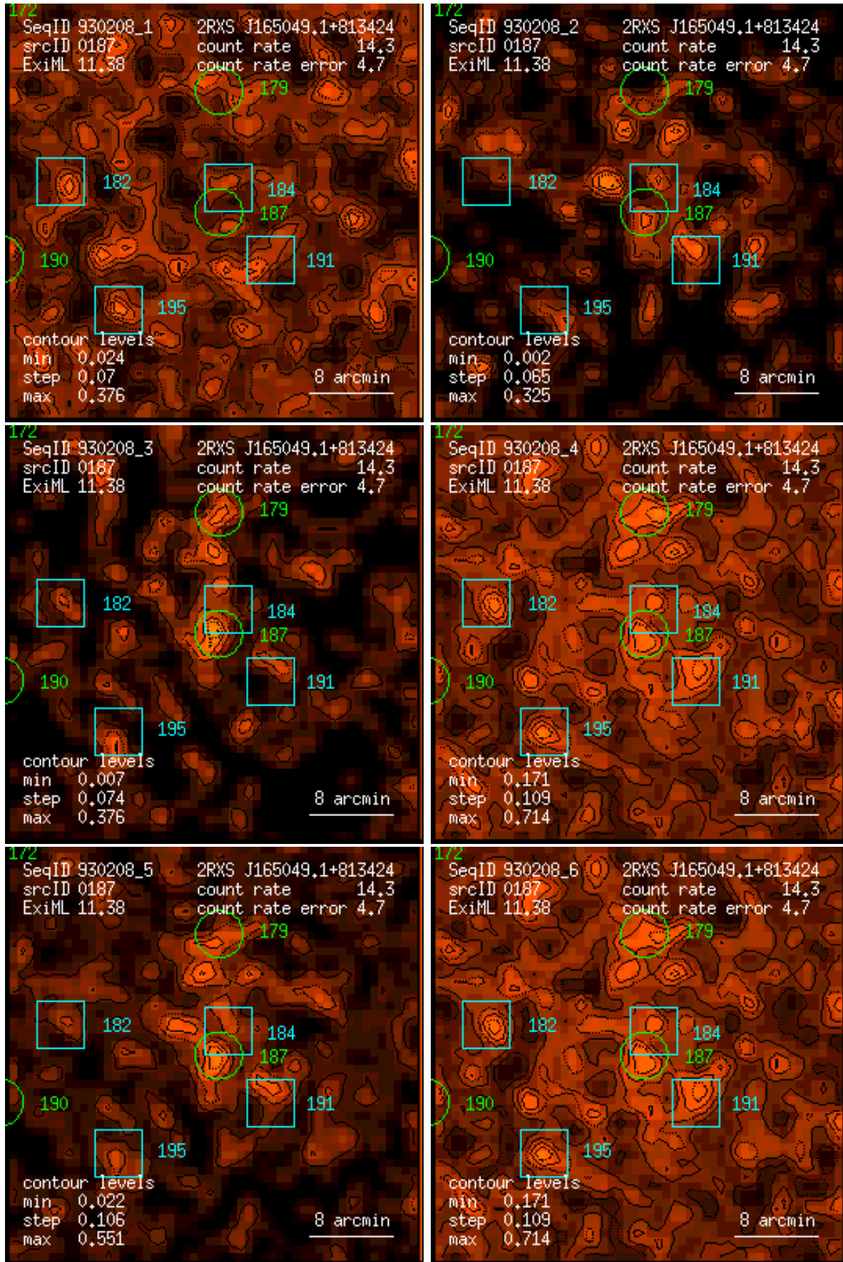
Figure 187: RASS 930208: detection 0187: band rate images, Gaussian filter: (1) PSPC channels 11 – 41, (2) 52 – 90, (3) 91 – 201, (4) 11 – 235, (5) 52 – 201, (6) 11 – 201. Broad band rates in counts/ks. Band rate contour levels in counts/ks/arcmin 2 .
