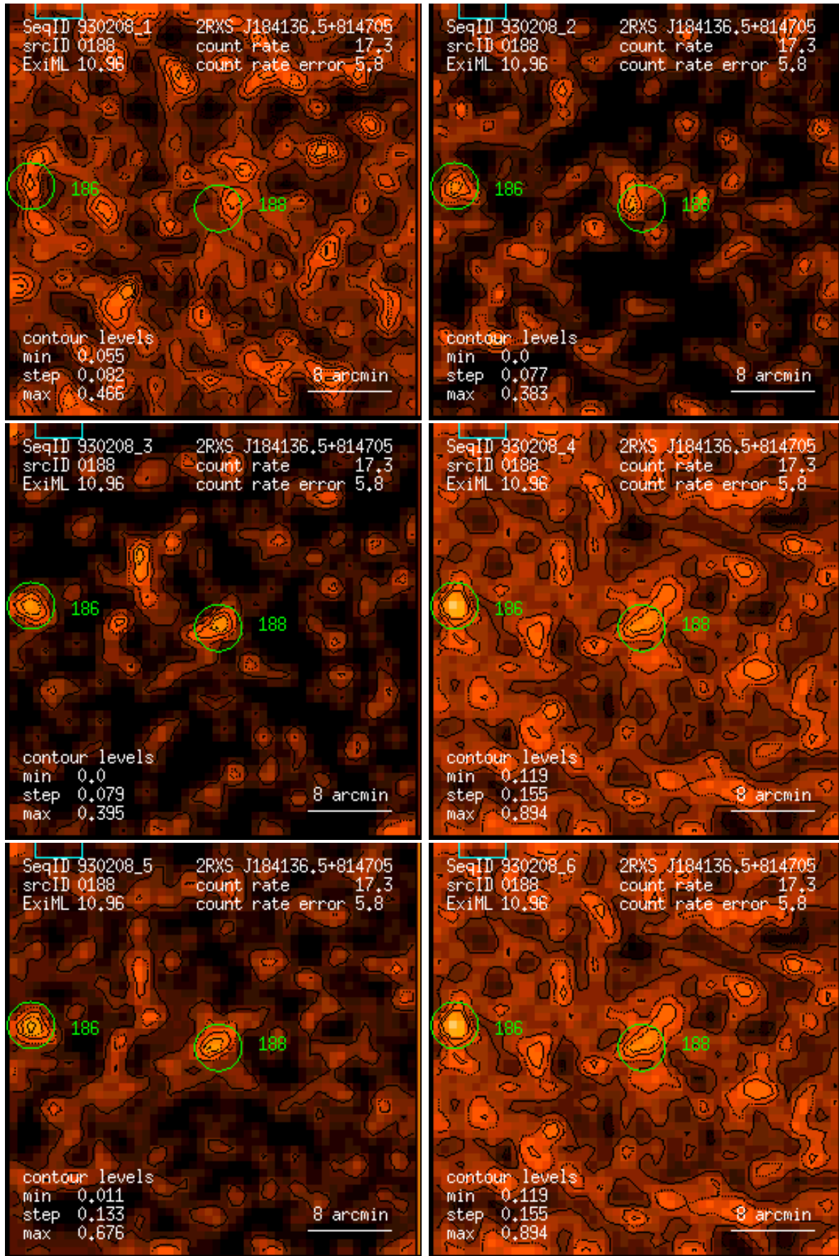
Figure 188: RASS 930208: detection 0188: band rate images, Gaussian filter: (1) PSPC channels 11 – 41, (2) 52 – 90, (3) 91 – 201, (4) 11 – 235, (5) 52 – 201, (6) 11 – 201. Broad band rates in counts/ks. Band rate contour levels in counts/ks/arcmin 2 .
