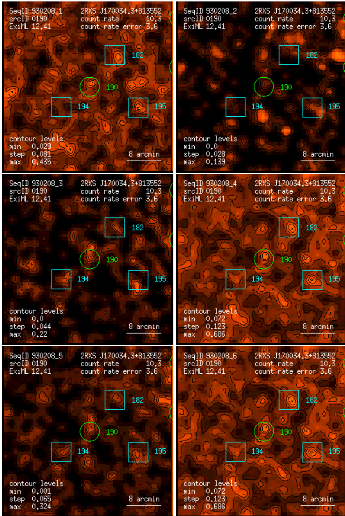
Figure 190: RASS 930208: detection 0190: band rate images, Gaussian filter: (1) PSPC channels 11 – 41, (2) 52 – 90, (3) 91 – 201, (4) 11 – 235, (5) 52 – 201, (6) 11 – 201. Broad band rates in counts/ks. Band rate contour levels in counts/ks/arcmin 2 .
