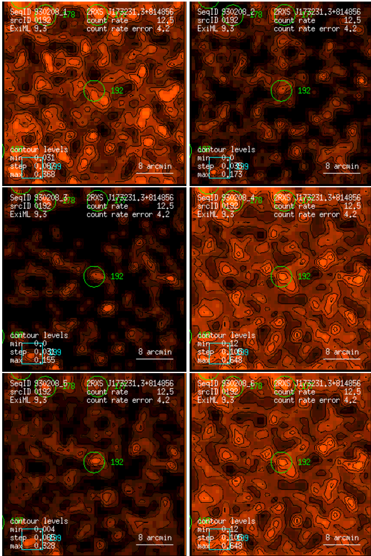
Figure 192: RASS 930208: detection 0192: band rate images, Gaussian filter: (1) PSPC channels 11 – 41, (2) 52 – 90, (3) 91 – 201, (4) 11 – 235, (5) 52 – 201, (6) 11 – 201. Broad band rates in counts/ks. Band rate contour levels in counts/ks/arcmin 2 .
