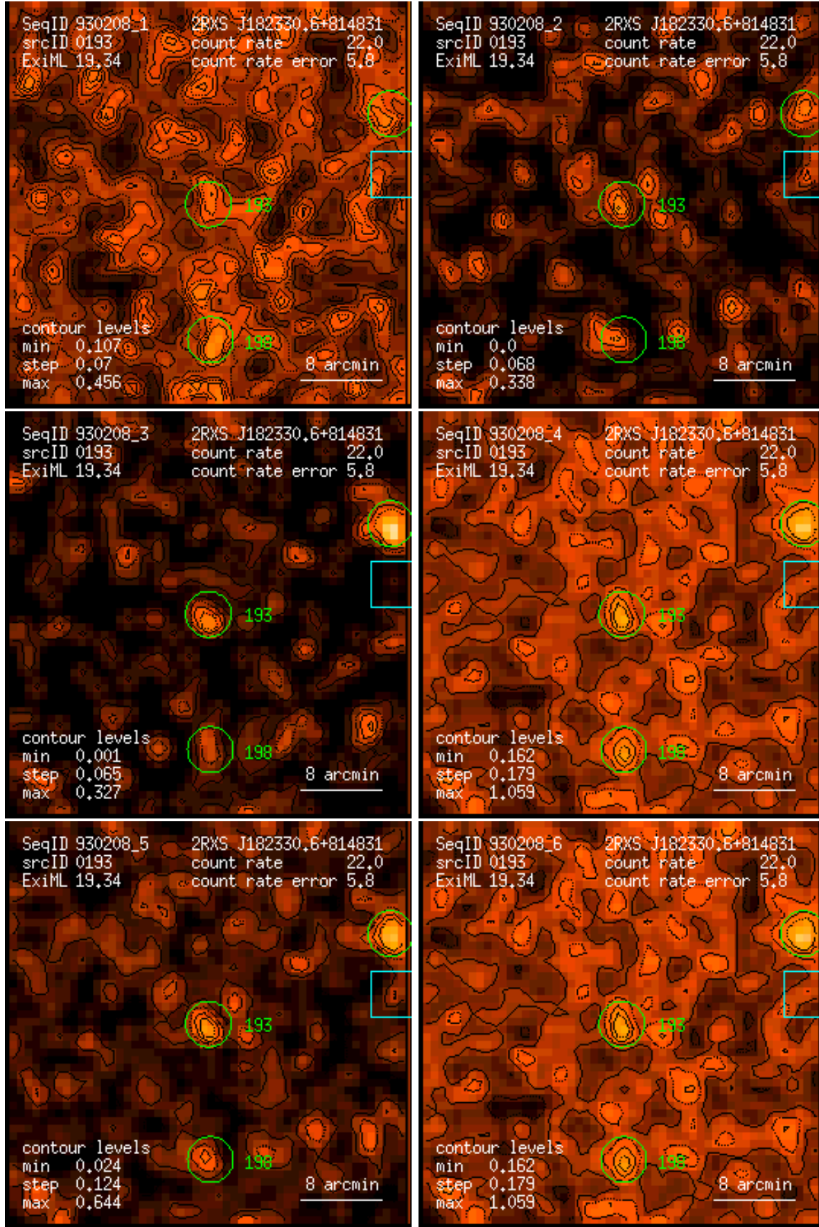
Figure 193: RASS 930208: detection 0193: band rate images, Gaussian filter: (1) PSPC channels 11 – 41, (2) 52 – 90, (3) 91 – 201, (4) 11 – 235, (5) 52 – 201, (6) 11 – 201. Broad band rates in counts/ks. Band rate contour levels in counts/ks/arcmin 2 .
