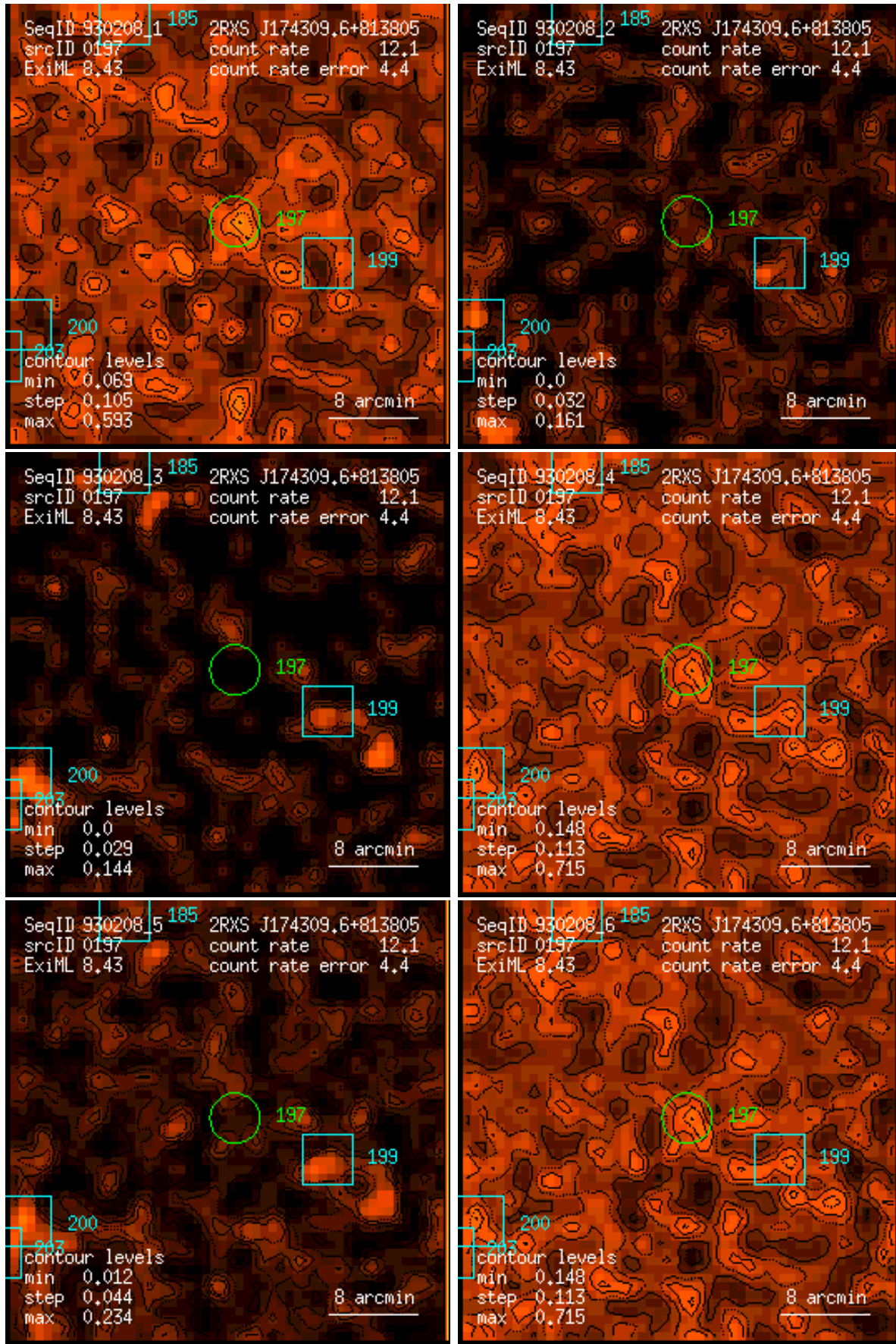
Figure 197: RASS 930208: detection 0197: band rate images, Gaussian filter: (1) PSPC channels 11 – 41, (2) 52 – 90, (3) 91 – 201, (4) 11 – 235, (5) 52 – 201, (6) 11 – 201. Broad band rates in counts/ks. Band rate contour levels in counts/ks/arcmin 2 .
