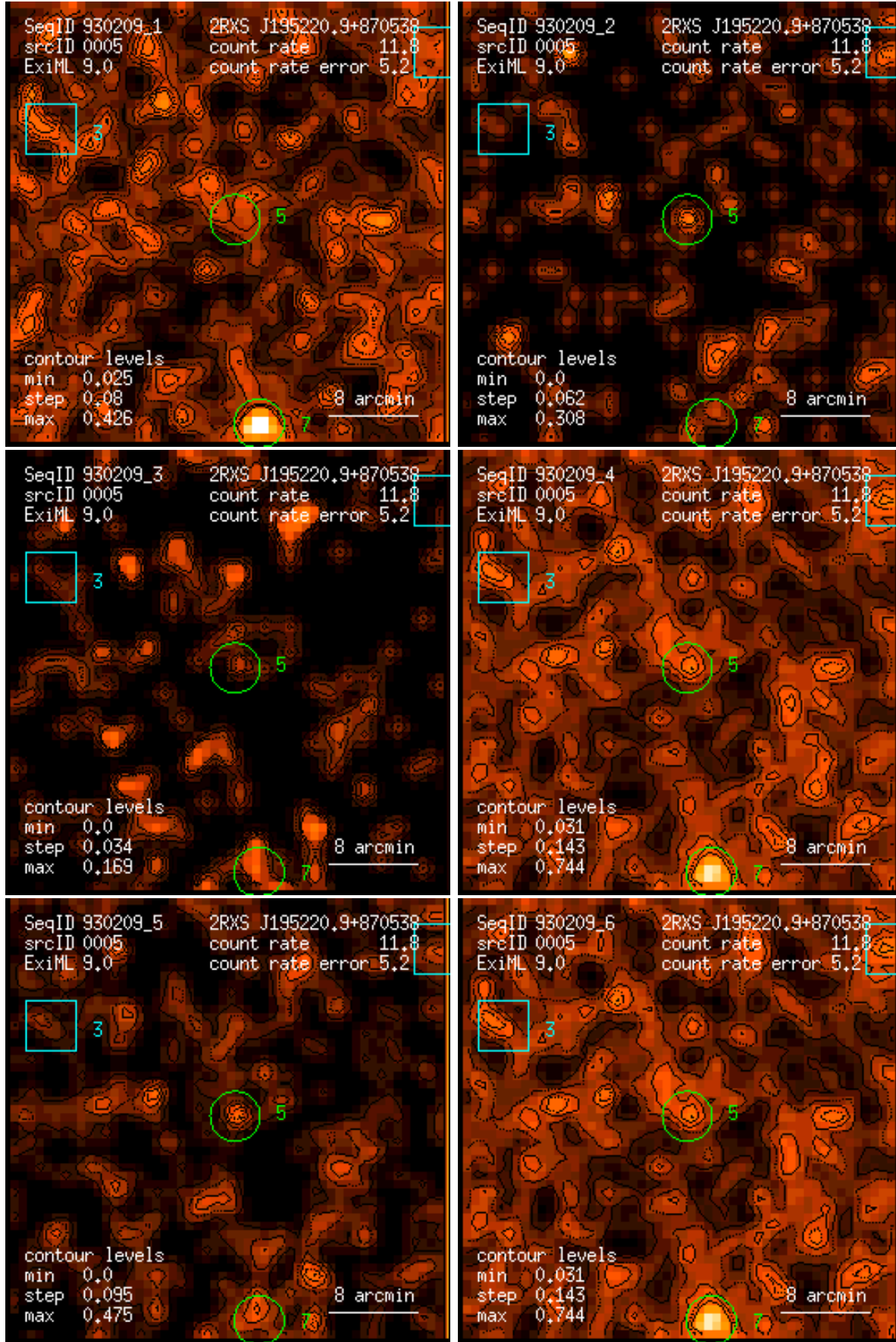
Figure 5: RASS 930209: detection 0005: band rate images, Gaussian filter: (1) PSPC channels 11 – 41, (2) 52 – 90, (3) 91 – 201, (4) 11 – 235, (5) 52 – 201, (6) 11 – 201. Broad band rates in counts/ks. Band rate contour levels in counts/ks/arcmin 2 .
