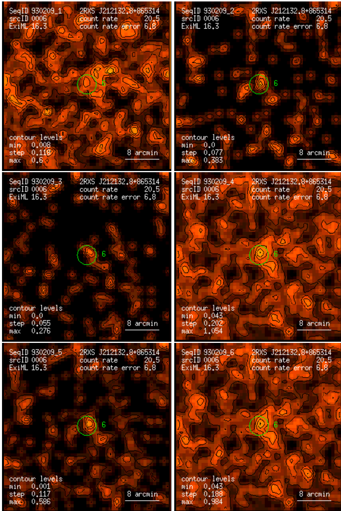
Figure 6: RASS 930209: detection 0006: band rate images, Gaussian filter: (1) PSPC channels 11 – 41, (2) 52 – 90, (3) 91 – 201, (4) 11 – 235, (5) 52 – 201, (6) 11 – 201. Broad band rates in counts/ks. Band rate contour levels in counts/ks/arcmin 2 .
