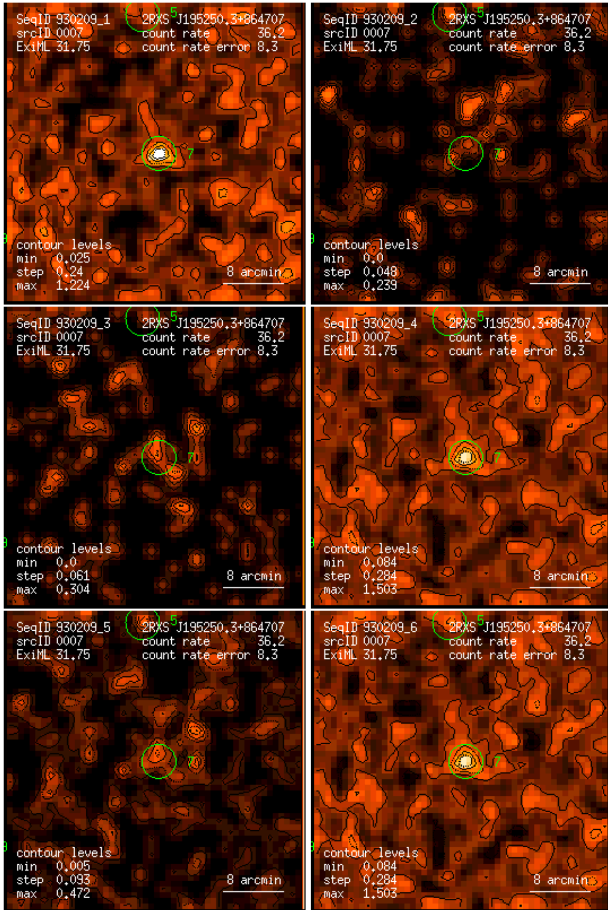
Figure 7: RASS 930209: detection 0007: band rate images, Gaussian filter: (1) PSPC channels 11 – 41, (2) 52 – 90, (3) 91 – 201, (4) 11 – 235, (5) 52 – 201, (6) 11 – 201. Broad band rates in counts/ks. Band rate contour levels in counts/ks/arcmin 2 .
