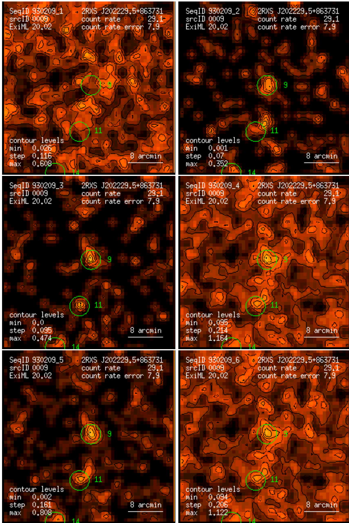
Figure 9: RASS 930209: detection 0009: band rate images, Gaussian filter: (1) PSPC channels 11 – 41, (2) 52 – 90, (3) 91 – 201, (4) 11 – 235, (5) 52 – 201, (6) 11 – 201. Broad band rates in counts/ks. Band rate contour levels in counts/ks/arcmin 2 .
