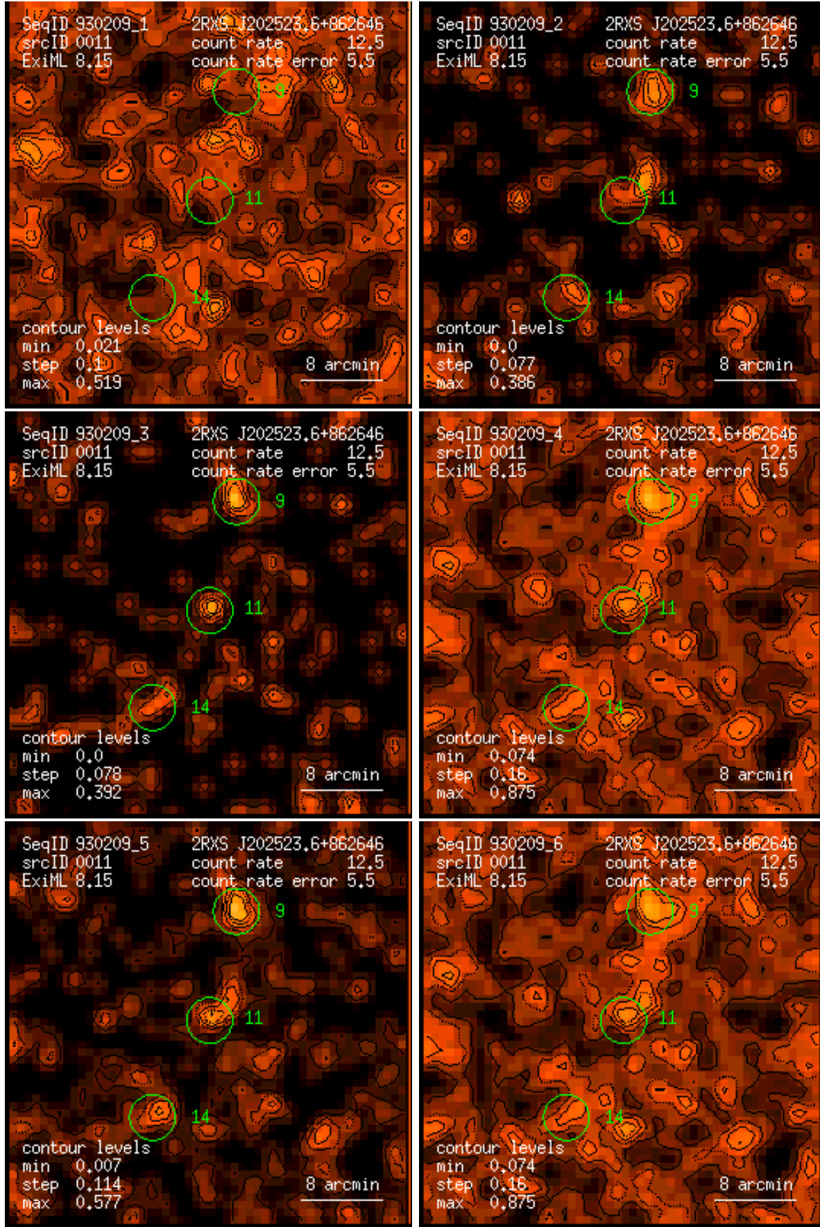
Figure 11: RASS 930209: detection 0011: band rate images, Gaussian filter: (1) PSPC channels 11 – 41, (2) 52 – 90, (3) 91 – 201, (4) 11 – 235, (5) 52 – 201, (6) 11 – 201. Broad band rates in counts/ks. Band rate contour levels in counts/ks/arcmin 2 .
