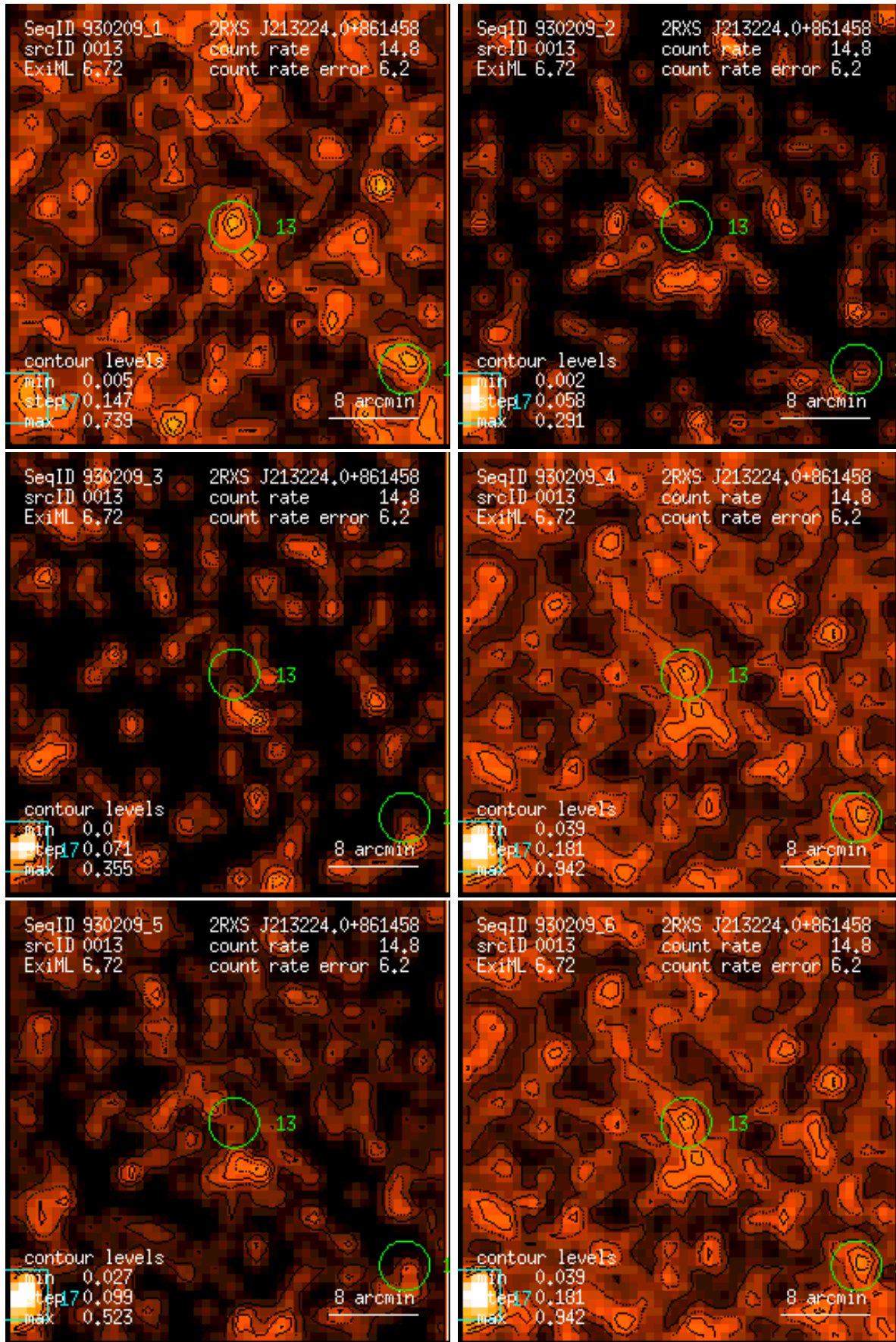
Figure 13: RASS 930209: detection 0013: band rate images, Gaussian filter: (1) PSPC channels 11 – 41, (2) 52 – 90, (3) 91 – 201, (4) 11 – 235, (5) 52 – 201, (6) 11 – 201. Broad band rates in counts/ks. Band rate contour levels in counts/ks/arcmin 2 .
