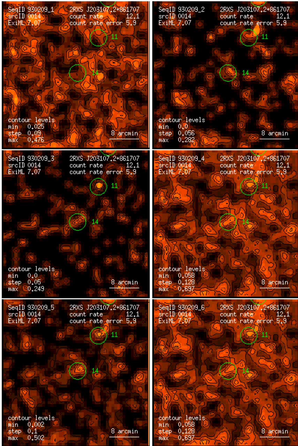
Figure 14: RASS 930209: detection 0014: band rate images, Gaussian filter: (1) PSPC channels 11 – 41, (2) 52 – 90, (3) 91 – 201, (4) 11 – 235, (5) 52 – 201, (6) 11 – 201. Broad band rates in counts/ks. Band rate contour levels in counts/ks/arcmin 2 .
