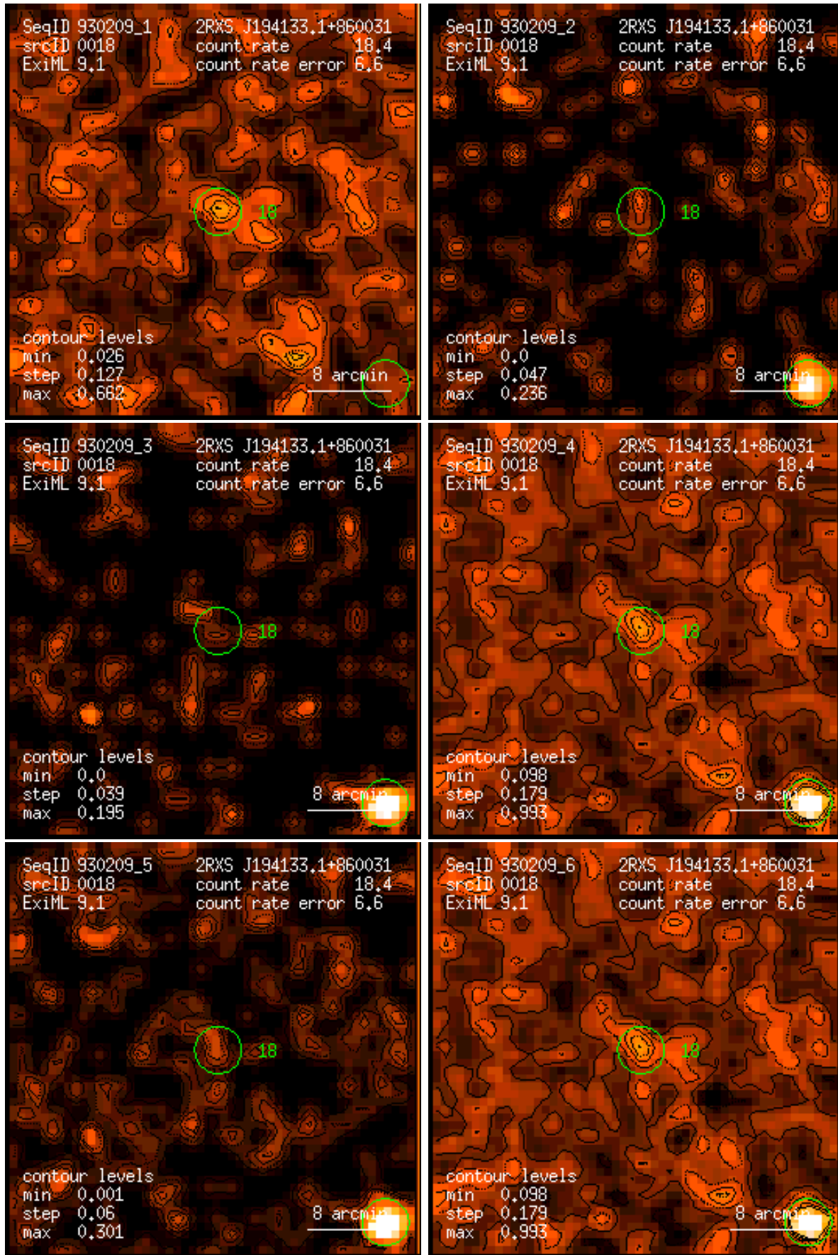
Figure 18: RASS 930209: detection 0018: band rate images, Gaussian filter: (1) PSPC channels 11 – 41, (2) 52 – 90, (3) 91 – 201, (4) 11 – 235, (5) 52 – 201, (6) 11 – 201. Broad band rates in counts/ks. Band rate contour levels in counts/ks/arcmin 2 .
