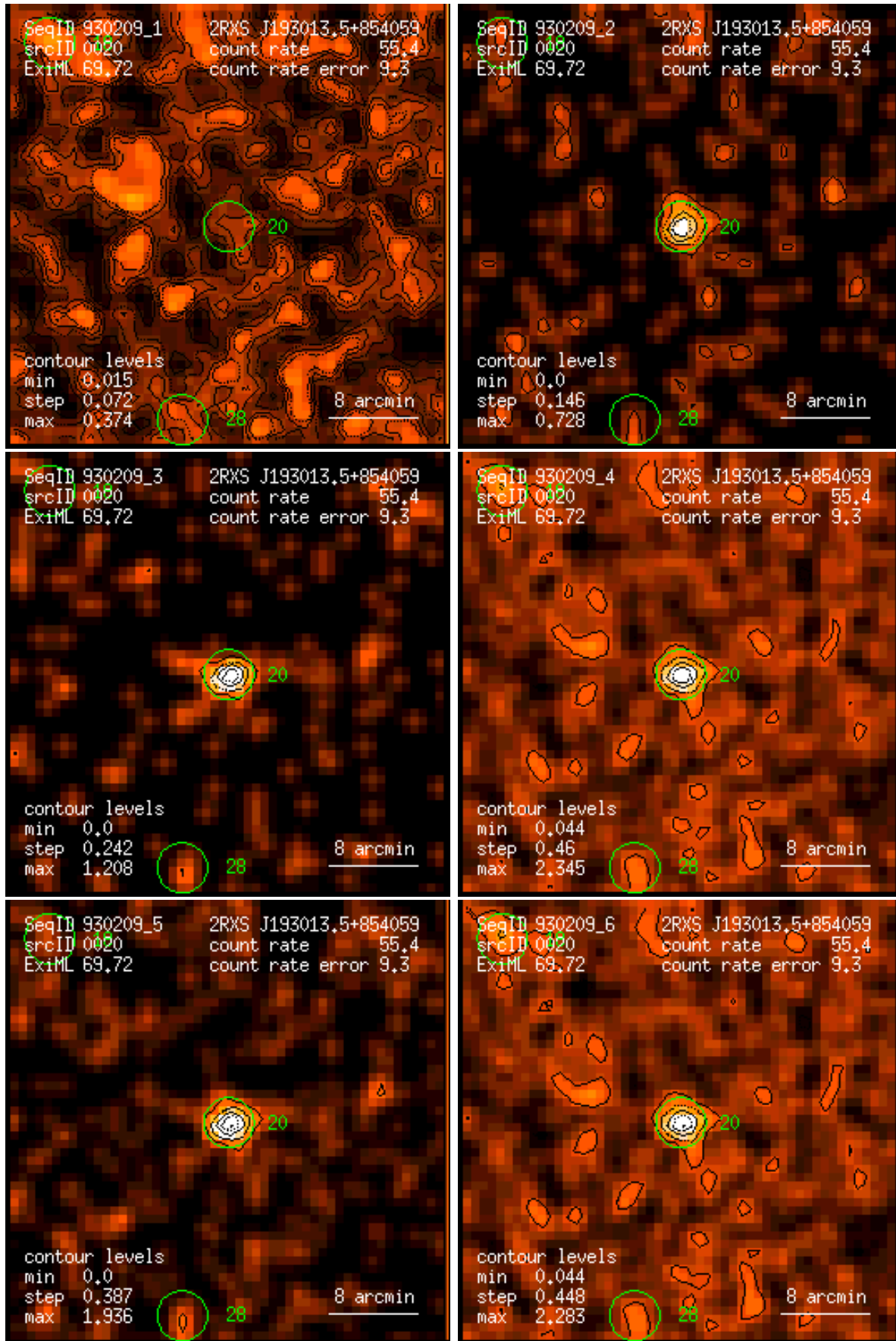
Figure 20: RASS 930209: detection 0020: band rate images, Gaussian filter: (1) PSPC channels 11 – 41, (2) 52 – 90, (3) 91 – 201, (4) 11 – 235, (5) 52 – 201, (6) 11 – 201. Broad band rates in counts/ks. Band rate contour levels in counts/ks/arcmin 2 .
