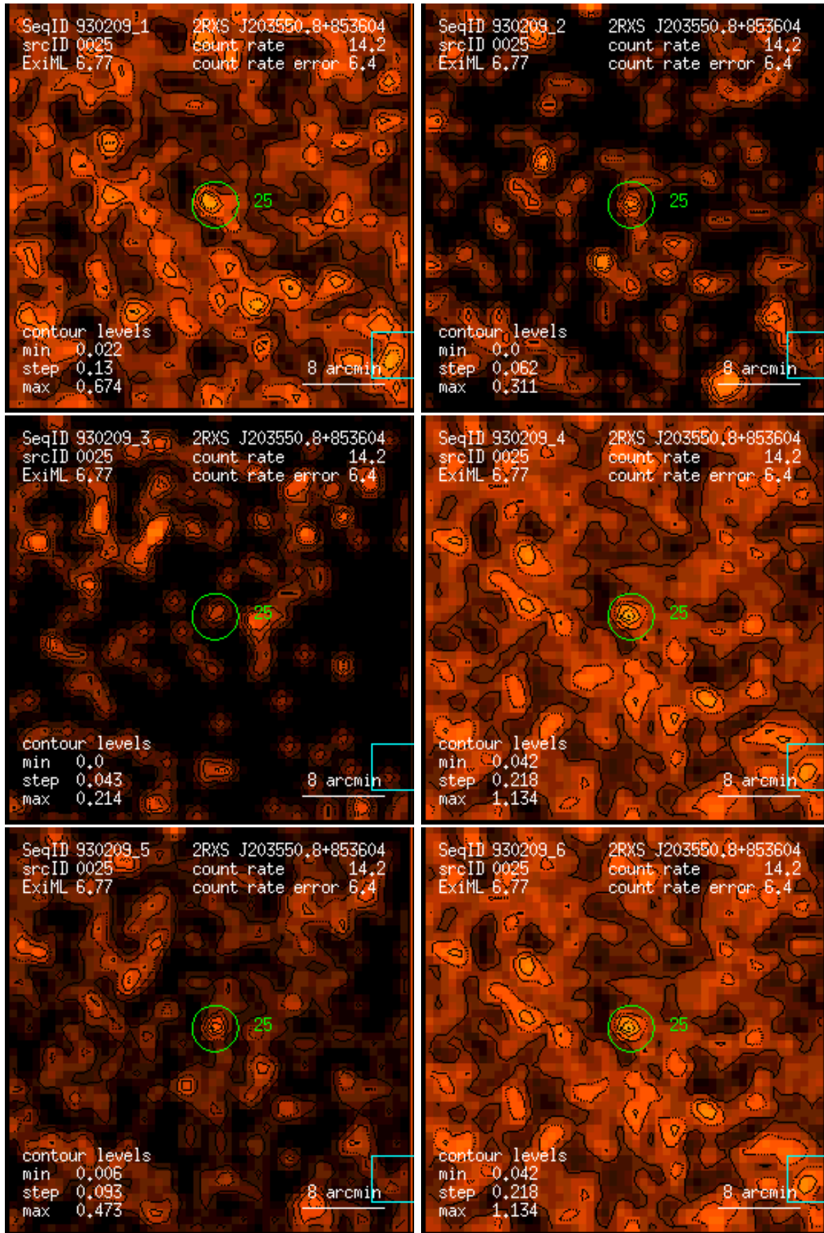
Figure 25: RASS 930209: detection 0025: band rate images, Gaussian filter: (1) PSPC channels 11 – 41, (2) 52 – 90, (3) 91 – 201, (4) 11 – 235, (5) 52 – 201, (6) 11 – 201. Broad band rates in counts/ks. Band rate contour levels in counts/ks/arcmin 2 .
