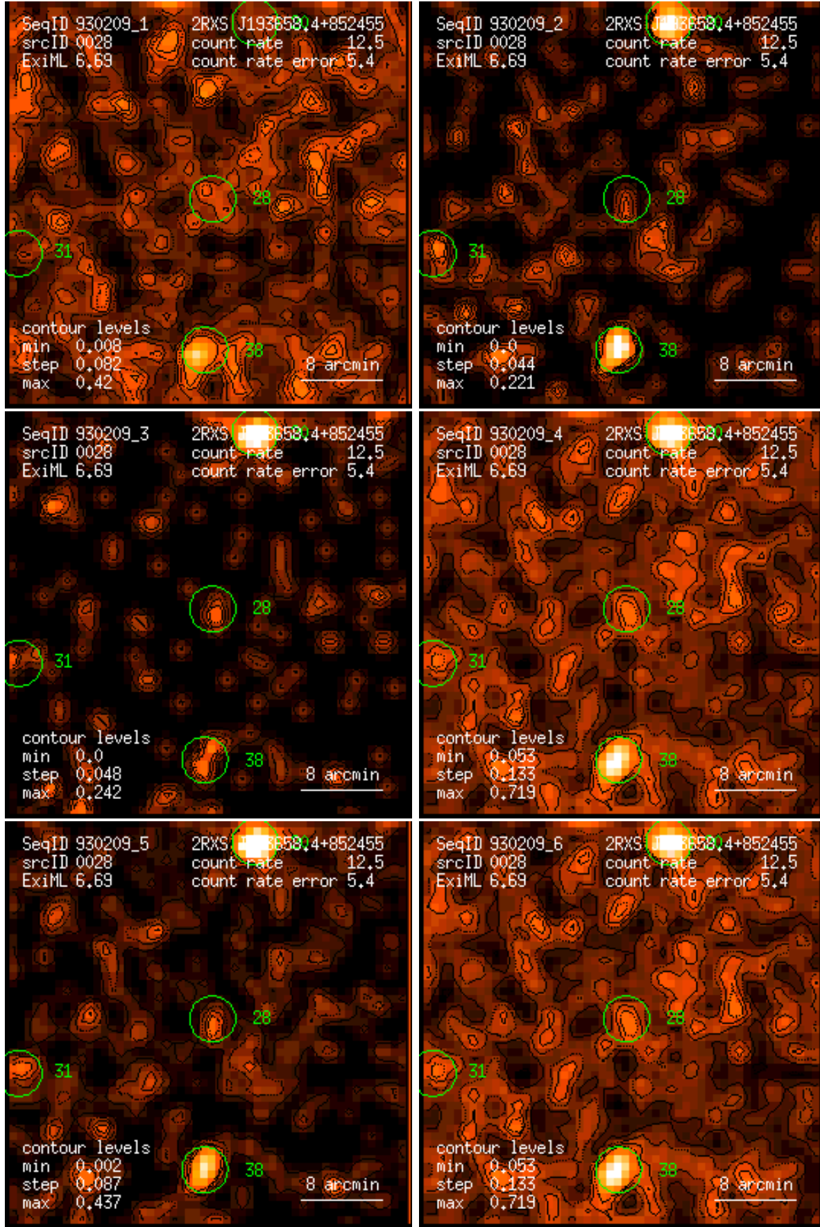
Figure 28: RASS 930209: detection 0028: band rate images, Gaussian filter: (1) PSPC channels 11 – 41, (2) 52 – 90, (3) 91 – 201, (4) 11 – 235, (5) 52 – 201, (6) 11 – 201. Broad band rates in counts/ks. Band rate contour levels in counts/ks/arcmin 2 .
