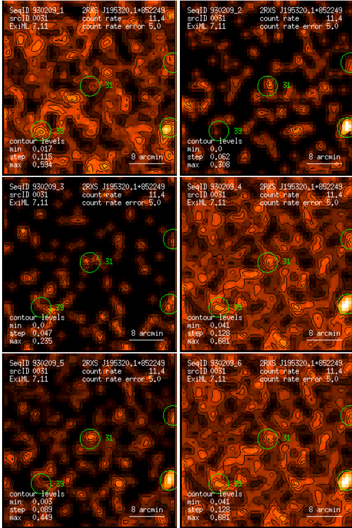
Figure 31: RASS 930209: detection 0031: band rate images, Gaussian filter: (1) PSPC channels 11 – 41, (2) 52 – 90, (3) 91 – 201, (4) 11 – 235, (5) 52 – 201, (6) 11 – 201. Broad band rates in counts/ks. Band rate contour levels in counts/ks/arcmin 2 .
