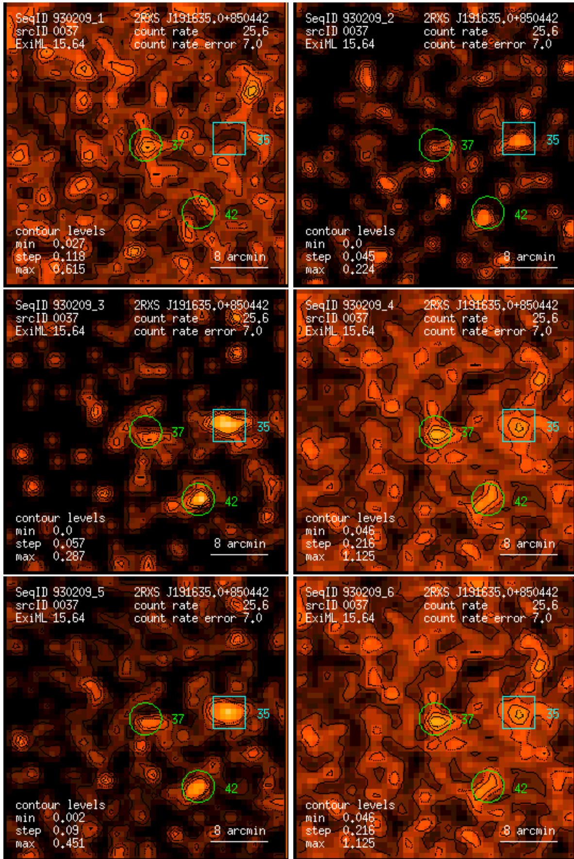
Figure 37: RASS 930209: detection 0037: band rate images, Gaussian filter: (1) PSPC channels 11 – 41, (2) 52 – 90, (3) 91 – 201, (4) 11 – 235, (5) 52 – 201, (6) 11 – 201. Broad band rates in counts/ks. Band rate contour levels in counts/ks/arcmin 2 .
