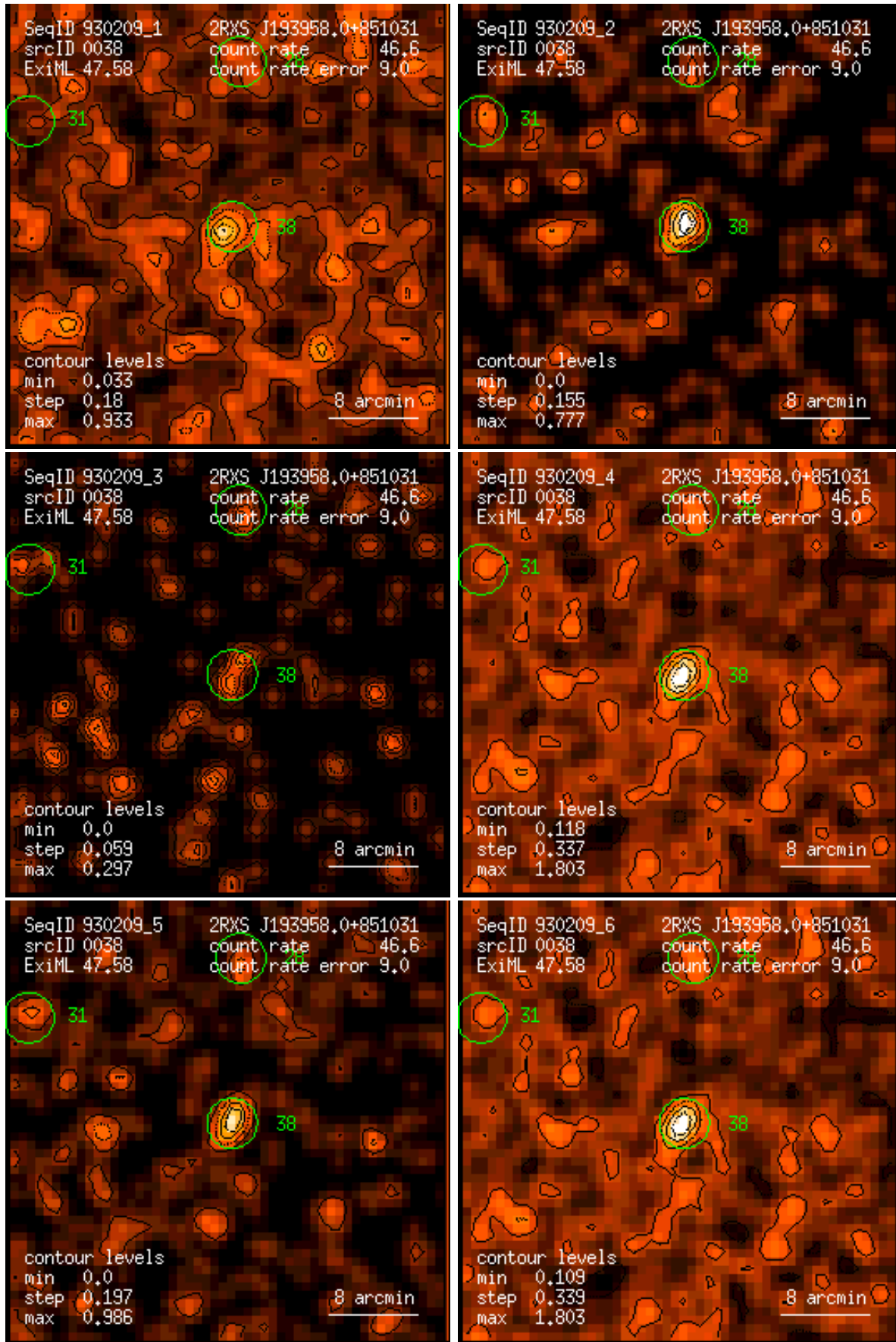
Figure 38: RASS 930209: detection 0038: band rate images, Gaussian filter: (1) PSPC channels 11 – 41, (2) 52 – 90, (3) 91 – 201, (4) 11 – 235, (5) 52 – 201, (6) 11 – 201. Broad band rates in counts/ks. Band rate contour levels in counts/ks/arcmin 2 .
